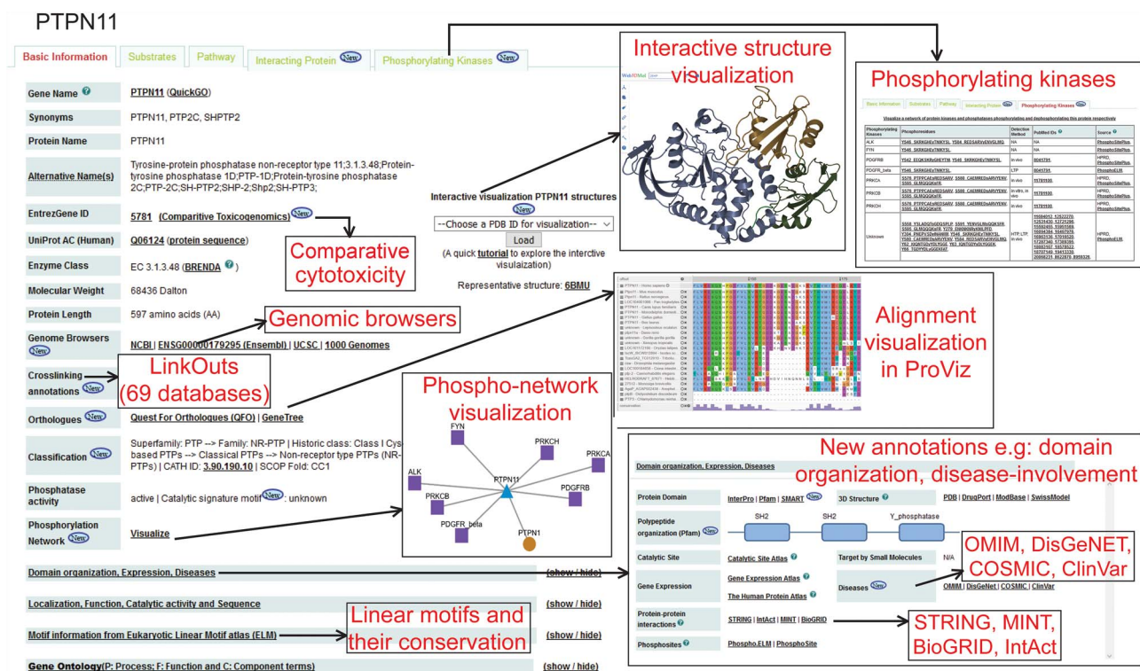
Figure 2. A typical protein entry in DEPOD. Various annotation fields are depicted and newly added annotations are highlighted separately. Phosphatase entries have a ‘Substrates’ tab that harbors information about its protein and non-protein substrates. Substrate entries have a ‘Phosphatases’ tab that includes information about phosphatases that dephosphorylate them.
