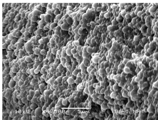
Figure 8. SEM micrograph of the poly(acrylamide) core matrix exhibiting the presence of poly(TPGDA-co-MMA) nanoparticles.
