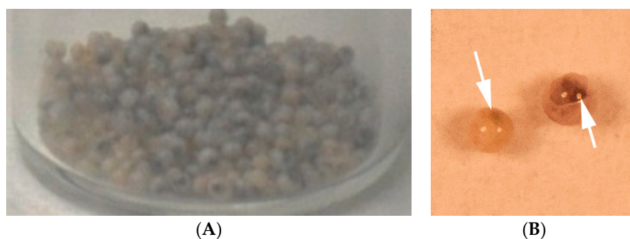
Figure 5. Optical image of dried composite/hybrid core-shell microparticles (A) and macro photography of two microparticles, the arrow point towards the reddish core (B).
