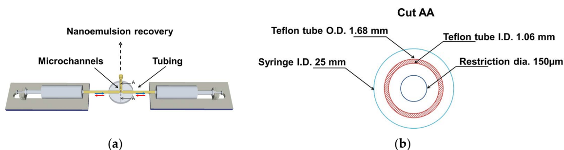
Figure 1. Schematic drawing of the microprocess to prepare the polymerizable nanoemulsion (not at scale, (a)), dimensions of the different channels in cut AA (b).
