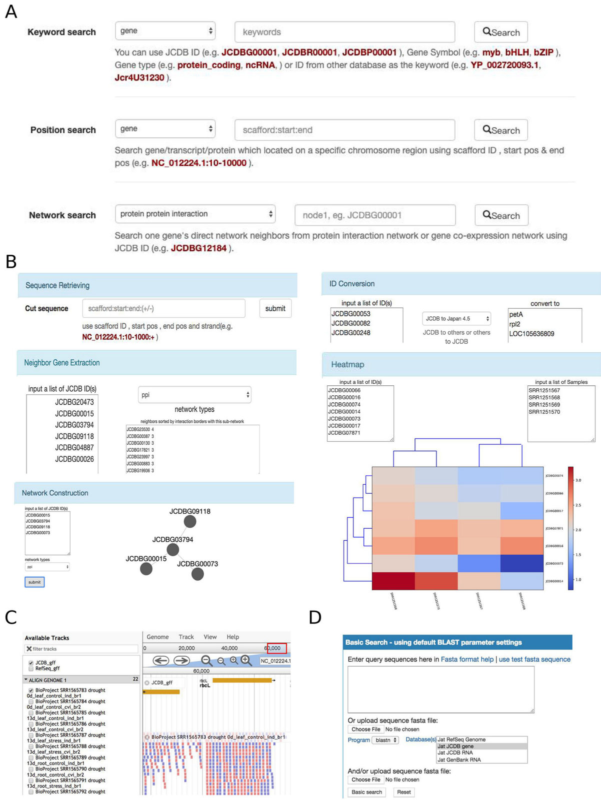
Fig. 2 Screenshots of the JCDB online tools. a Keyword search, position search, and network search. b JCDBtools, the web-based toolkit. c JBrowse, the genome browser. d Online BLAST search
