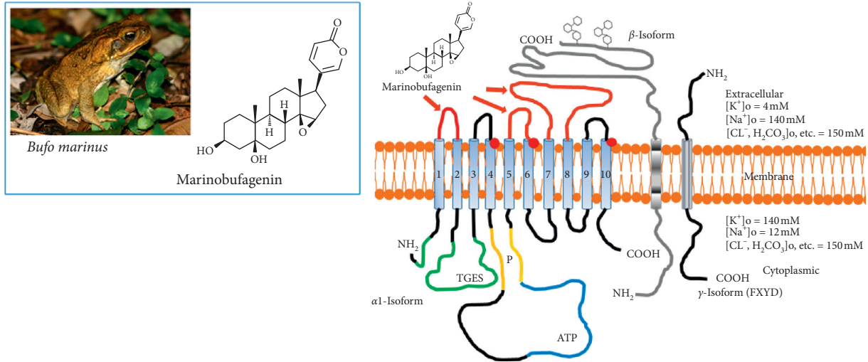
FIGURE 1: Chemical structures of bufadienolide, marinobufagenin and its pharmacological target, Na/K-ATPase.
