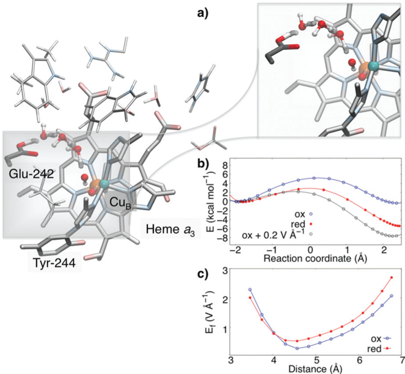
Fig. 4. PCET in cytochrome c oxidase. Reduction of the heme a_3/Cu_B leads to pT from Glu-242 via a water-chain to Cu_B ( Cu^{II}-OH^- ). (a) Close-up of the water-mediated pT reaction, (b) energy profiles for the pT reaction in the oxidised ( P_M ) and reduced ( P_R ) states, and the oxidised state upon application of a 0.2 V Å ^{-1} external field aligned along the pT direction, (c) computed electric fields for the oxidised ( P_M ) and reduced ( P_R ) states.
