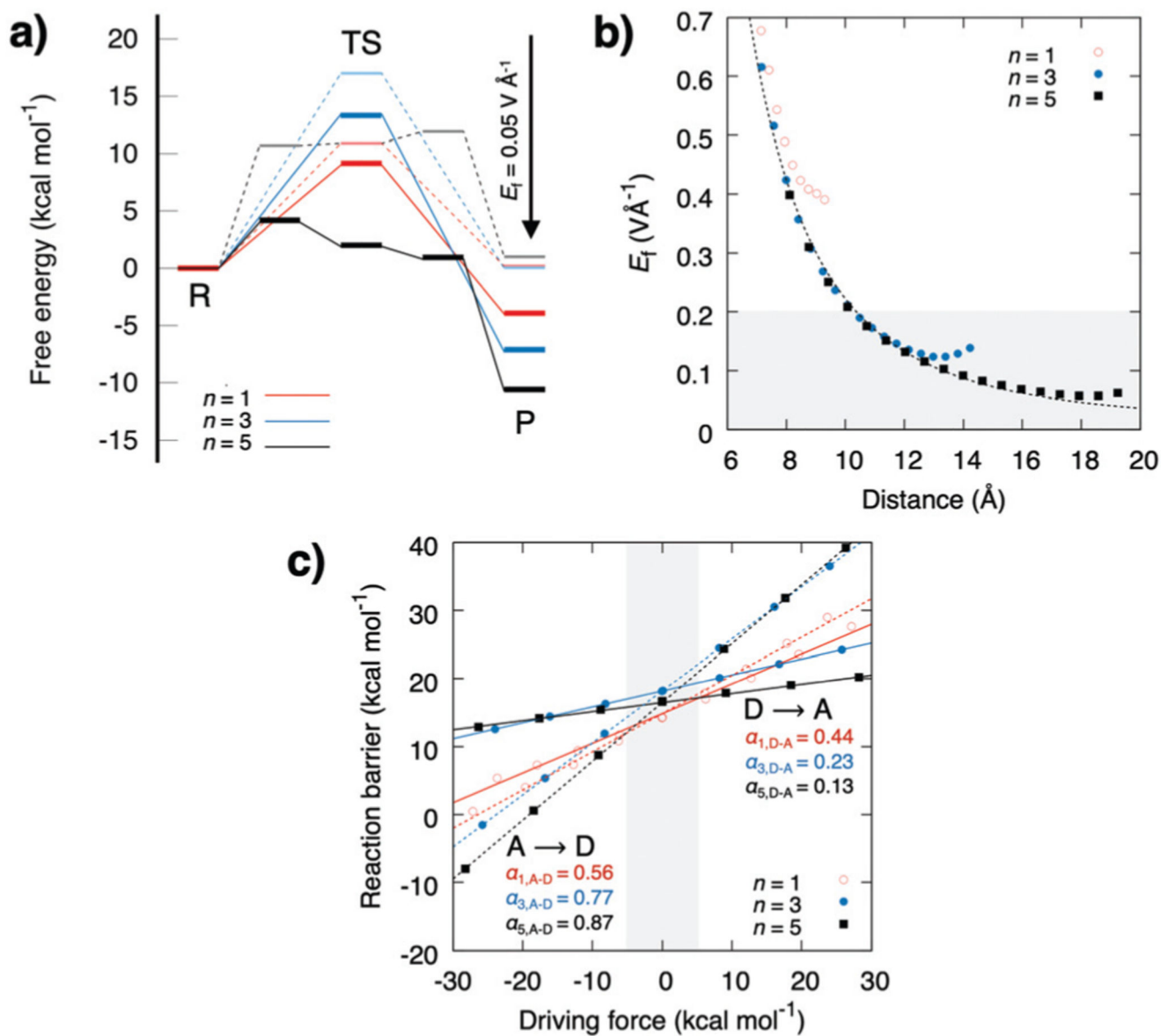
Fig. 3. (a) Effect of pT free energy profiles upon application of a uniform 0.05 \text{ V } \text{Å}^{-1} redox-field. (b) The electric field created by a redox reaction as a function of distance to the redox site, and (c) linear energy relationships between the thermodynamic driving force and the reaction barrier.
