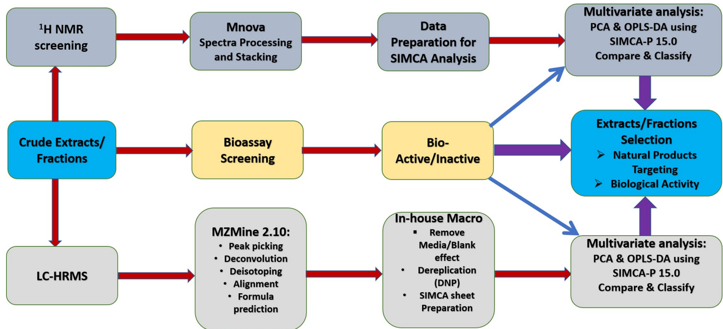
Fig 1. Metabolomics workflow chart to aid isolates selection.
