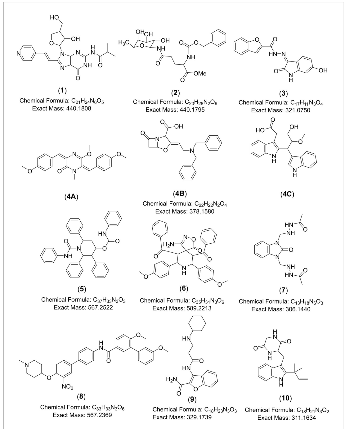
Fig 7. Chemical structures of dereplicated bioactive metabolites for the selected isolates MS.REE. 3, 6, 13 and 22.
