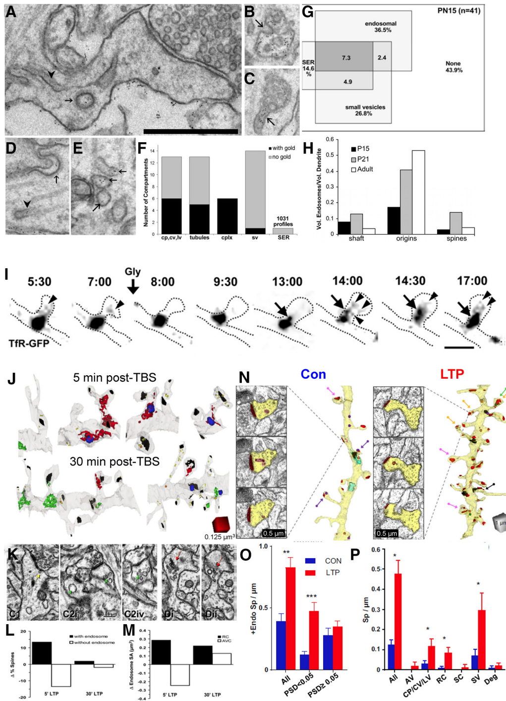
Figure 9. Endosomes move into dendritic spines in response to stimulation. A–E , Electron micrographs from a P21 hippocampal slice that was first given tetanic stimulation, followed by 900 pulses in the presence of bovine serum albumin conjugated to gold particles. A–E , Postsynaptic endocytosis was demonstrated by gold particles taken up from the extracellular space into large vesicles ( A ), invaginations into multivesicular bodies ( B ), sorting complexes with tubules ( C ), coated pits ( D ), and amorphous vesicular clumps ( E ). F , Quantification of gold particles in coated pits (cp), tubules, and sorting complexes (cplx). Note that particles were rarely seen in small presumably exocytic postsynaptic vesicles (sv), and never in SER profiles. G , Venn diagram representing the relative distribution of the named subcellular compartments occupying dendritic spines at postnatal day 15 of a total of 41 dendritic spines. H , Relative distribution of endosomal compartments in the dendritic shafts, at the origins of spines, and inside dendritic spine necks or heads for three developmental stages. A–H are adapted from Cooney et al. (2002). I , Time-lapse imaging of recycling endosomes mobilized into spines after glycine stimulation. Neurons expressing GFP-tagged transferrin receptor (TfR-GFP), a classic recycling cargo, and monomeric red fluorescent protein to fill the spines, represented by the dotted line. The spines were imaged every 15–30 s before and after glycine stimulation (200 mM, 3 min). Times are indicated as minutes:seconds. Arrows indicate the movement of large endosomes into the spine from the shaft. Arrowheads indicate vesicles or tubules emanating from larger TfR-containing endosomes. Scale bars, 1 μm. J , 3DEM reconstructions of dendritic segments at 5 and 30 min after TBS illustrating endosomes occupying the shaft and spines. (PSDs are in black; red, green, and blue represent different endosomal compartments). K , Example dendritic protrusions with large vesicular components. L , Changes in the percentages of spines with endosomes after LTP induction. M , Change in the amount of surface area available in the endosomes. I–M are adapted from Park et al. (2006). N , Electron micrographs and 3D reconstructions of dendritic segments illustrating the increase in the number of small spines at 2 h after the induction of LTP. O, P , Increased occupancy of endosomes in small spines 2 h after LTP. N and O are adapted from Kulik et al. (2019). * p < 0.05 ; ** p < 0.01 ; *** p < 0.001 .
