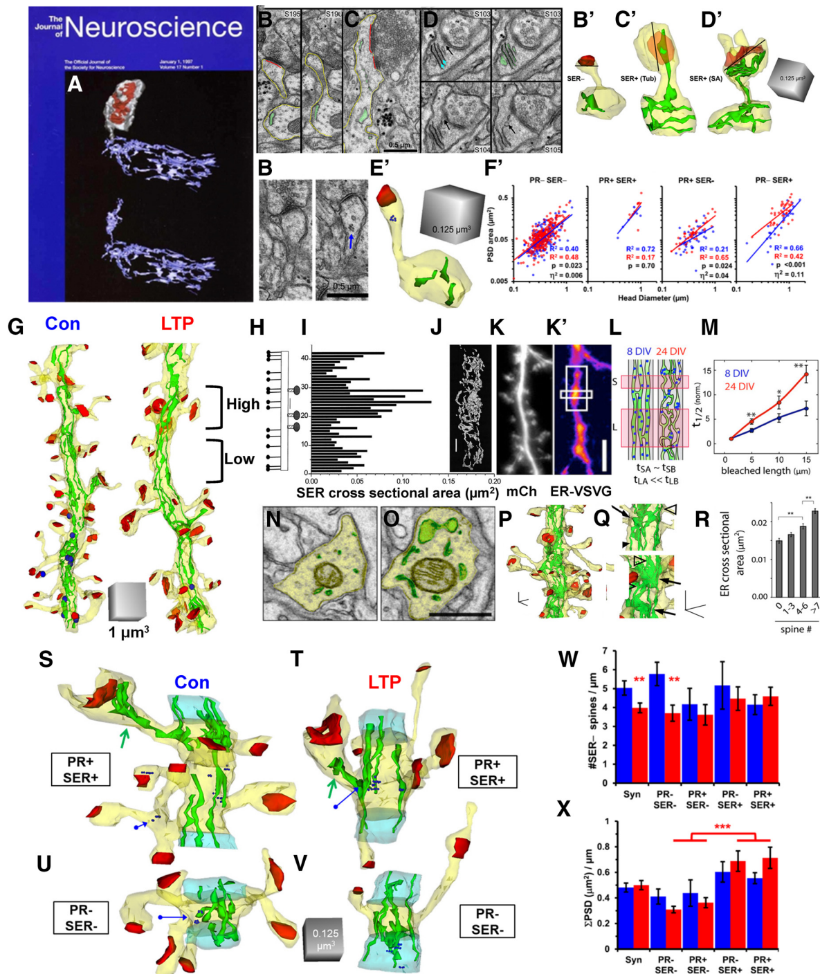
Figure 8. Effects of SER and PRs on synaptic plasticity and homeostasis. A , Three-dimensional reconstruction of a large dendritic spine (gray), with a large, irregular, perforated synapse (red) and its spine apparatus, which is continuous with the network of SER in the dendritic shaft. B–D' , Serial EM sections and three-dimensional reconstructions of spines: a spine without SER ( B, B' ), a spine with a simple tubule of SER ( C, C' ), and a spine with a spine apparatus ( D, D' ). The lines in the 3D reconstructions illustrate how the head diameter was measured at its widest point. E, E' , Serial sections and 3DEM illustrating a polyribosome in an adult dendritic spine head (blue arrow). F, F' , Synapse enlargement after LTP, controlled for head diameter relative to subcellular composition. G , Fully reconstructed dendritic segments from adult rat hippocampal slices under control (Con) and LTP conditions, illustrating regions of high and low spine density. H, I , In adult hippocampus in vivo , the schematic shows the locations of small and large spine origins ( H ), which match the section locations indicated in I , where the y -axis is the section number and the x -axis charts the total cross-sectional area of SER in the dendritic shaft on each segment. J , 3DEM of the shaft SER that is graphed in I . K–L , In cultured hippocampal dendrites, we showed that where the dendritic shaft SER was more complex in structure, trafficking was slowed and provided regions for cargo exit to deliver resources to synapses. M , The length of the complex ER exit sites increased with age. N–R , Regions of SER complexity gave rise to more dendritic spines in adult hippocampus. S, T , Synaptic clusters having spines with large synapses and resource rich spines containing polyribosomes or SER (PR + , SER + ) in the control (Con) and LTP conditions. U, V , Synaptic clusters lacking resource-rich dendritic spines (PR − , SER − ) in the control and LTP conditions. W , The homeostatic stalling of spine outgrowth was restricted to synaptic clusters lacking resource-rich spines. X , In contrast, regions of the dendritic segment that had resource-rich spines had a greater total synaptic weight, measured as the summed PSD area per length of cluster segment. A and H–J are adapted from Spacek and Harris (1997); B–G and S–X are adapted from Chirillo et al. (2019); K–R are adapted from Cui-Wang et al. (2012).
