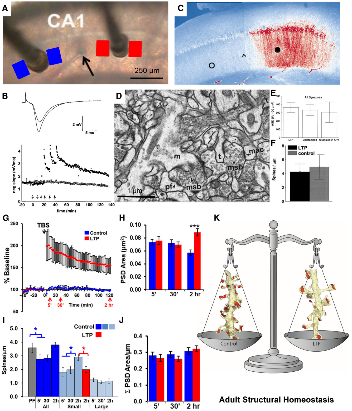
Figure 5. Ultrastructure of long-term potentiation in the young adult rat hippocampus. A , Positioning of stimulating electrodes and sample locations for serial EM sections from the control (blue) and LTP (red) sites. The stimulating electrode that induced LTP was alternated between the CA3 (left) and the subicular (right) side of the recording electrode (black arrow). B , LTP induced by three bouts of tetanic stimulation (closed arrows, 100 Hz for 1 s each), and the control side received the same number of stimuli at a slower rate that did not induce LTP (open arrows). C , Staining for P-CaMKII after induction of LTP at the subicular stimulating electrode (black circle) illustrates increased labeling (red) of P-CaMKII relative to the control stimulation site (open circle). The arrowhead indicates the approximate location of the recording electrode, and the scale is the same as in A . Adapted from Ouyang et al. (1997). D , Illustration of the excellent brain slice ultrastructure that can be obtained from adult hippocampal slices. E, F , Examination of such slices revealed that adjusted synaptic density (ASD; E ) and spines per micrometer ( F ) were not altered by LTP induced by tetanic stimulation B and D–F were adapted from Sorra and Harris (1998). G–I , When LTP was induced with theta burst stimulation ( G ), and the PSD area of synapses enlarged ( H ), while the increase in small-spine density seen under control conditions was absent ( I ). J, K , Consequently, the total PSD area after LTP induction was similar to that in control conditions ( J ), resulting in a homeostatic balance in total synaptic weight per unit length of dendrite ( K ). A, B, G , and H are adapted from Bourne and Harris (2011); I is adapted from Bell et al. (2014). msb, Multisynaptic bouton. ( D ) m = mushroom spine, pf = perforated PSD, msb = multisynaptic bouton, mac = macular PSD, t = thin spine; * p < 0.05; *** p < 0.001.
