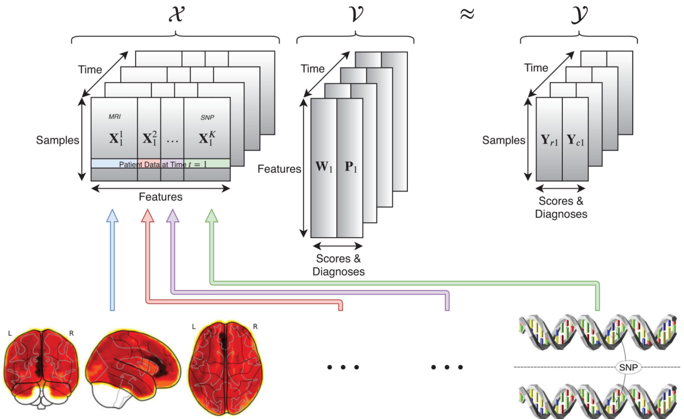
Fig. 1. Visualization of the input ( X ), coefficient ( V ) and output ( Y ) tensors. In each time-point of X the K modalities (MRI, SNP, etc.) are explicitly defined to facilitate the calculation of the group l_1 -norm. The goal of the proposed method is to learn a joint model V that can effectively map X to the cognitive scores and diagnoses encoded in Y .
