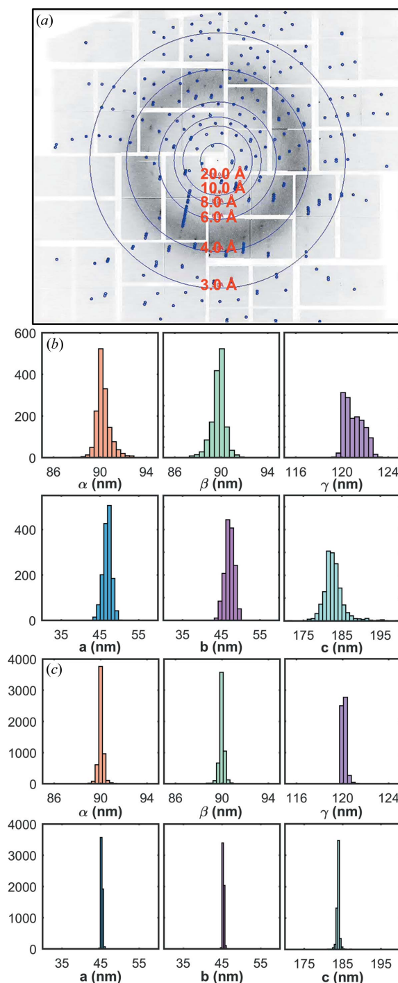
Figure 2 (a) REP24 microcrystals diffract up to ~2.2 Å. No degradation of resolution was observed as the exposure time to vacuum increased. (b) Histograms of unit-cell parameters from ~1400 indexed patterns in vacuum and (c) ~5500 indexed patterns in humidified helium.
