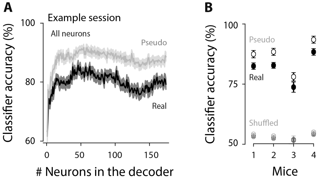
Figure 7. Noise correlations reduce classification accuracy. A , Classification accuracy for an example session (0-97 ms before the choice) on neural ensembles of increasingly larger size. Mean±SEM (50 cross-validated samples). Gray: classification accuracy for pseudo-populations. Black: real populations. Both cell types were included (“All neurons”). B , Summary for each mouse; points show mean±SEM across days. Values were computed for the largest neuronal ensemble (the max value on the horizontal axis in A ).
