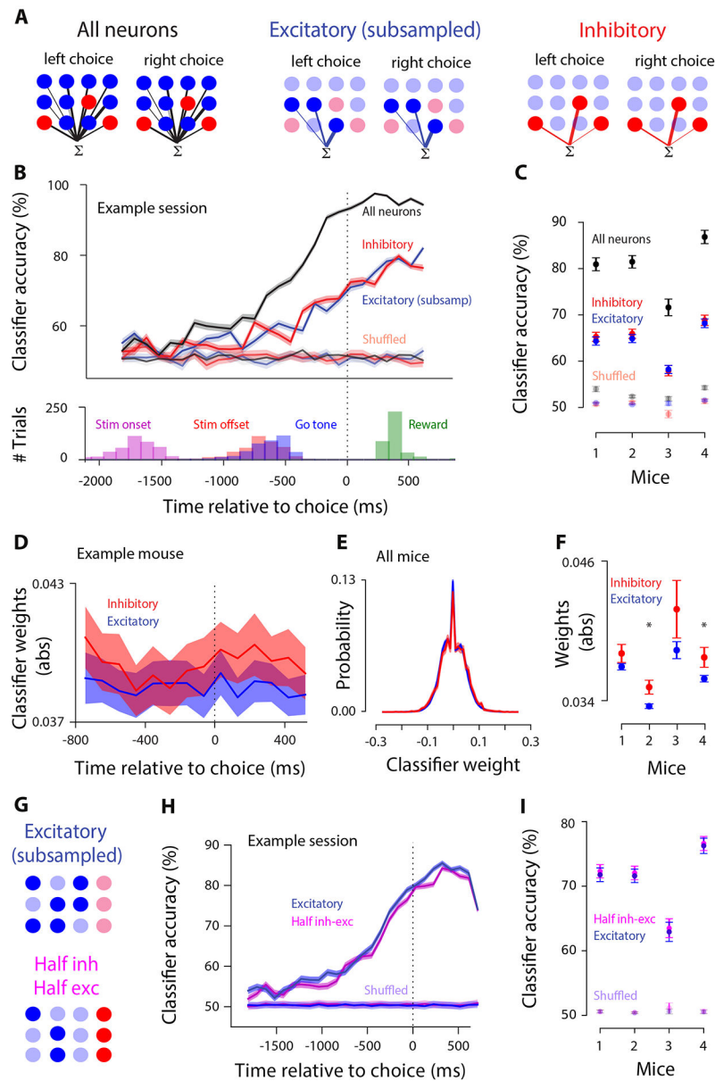
Figure 3. Linear classifiers can predict the animal's choice with equal accuracy from the activity of excitatory or inhibitory populations.
