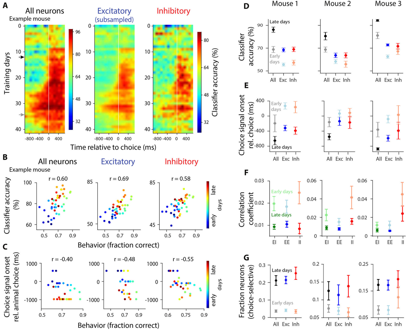
Figure 8. Learning leads to improved choice decoding, increased fraction of choice-selective neurons, and reduced noise correlations in both populations. A , Decoder accuracy for each training session, for all neurons (left), subsampled excitatory (middle), and inhibitory neurons (right). White vertical line: choice. Rows: average across cross-validated samples; example mouse. Colorbar applies to both plots. B , Scatter plot of classifier accuracy (0-97 ms before choice) vs. behavioral performance (fraction correct on easy trials) for all training days. r : Pearson correlation coefficient ( p < 0.001 in all plots); same example mouse as in (A). Correlations for behavior vs. classification accuracy for all neurons, excitatory and inhibitory: 0.55, 0.35, 0.32 in mouse 2; 0.57, 0.63, 0.32 in mouse 3. Correlations for behavior vs. choice-signal onset for all neurons, excitatory and inhibitory: -0.60 , -0.34 , -0.38 , in mouse 2; -0.60 , -0.27 , -0.28 in mouse 3. All values: p < 0.05 . C , Same as (B), except showing the onset of choice signal (the first moment in the trial that classifier accuracy was above chance, relative to choice onset) vs. behavioral performance. D , Summary of classification accuracy averaged across early (dim colors) vs. late (dark colors) training days. E , Same as (D), but showing choice signal onset (ms). F , Same as (D), but showing pairwise noise correlation coefficients. EI:excitatory-inhibitory; EE:excitatory-
