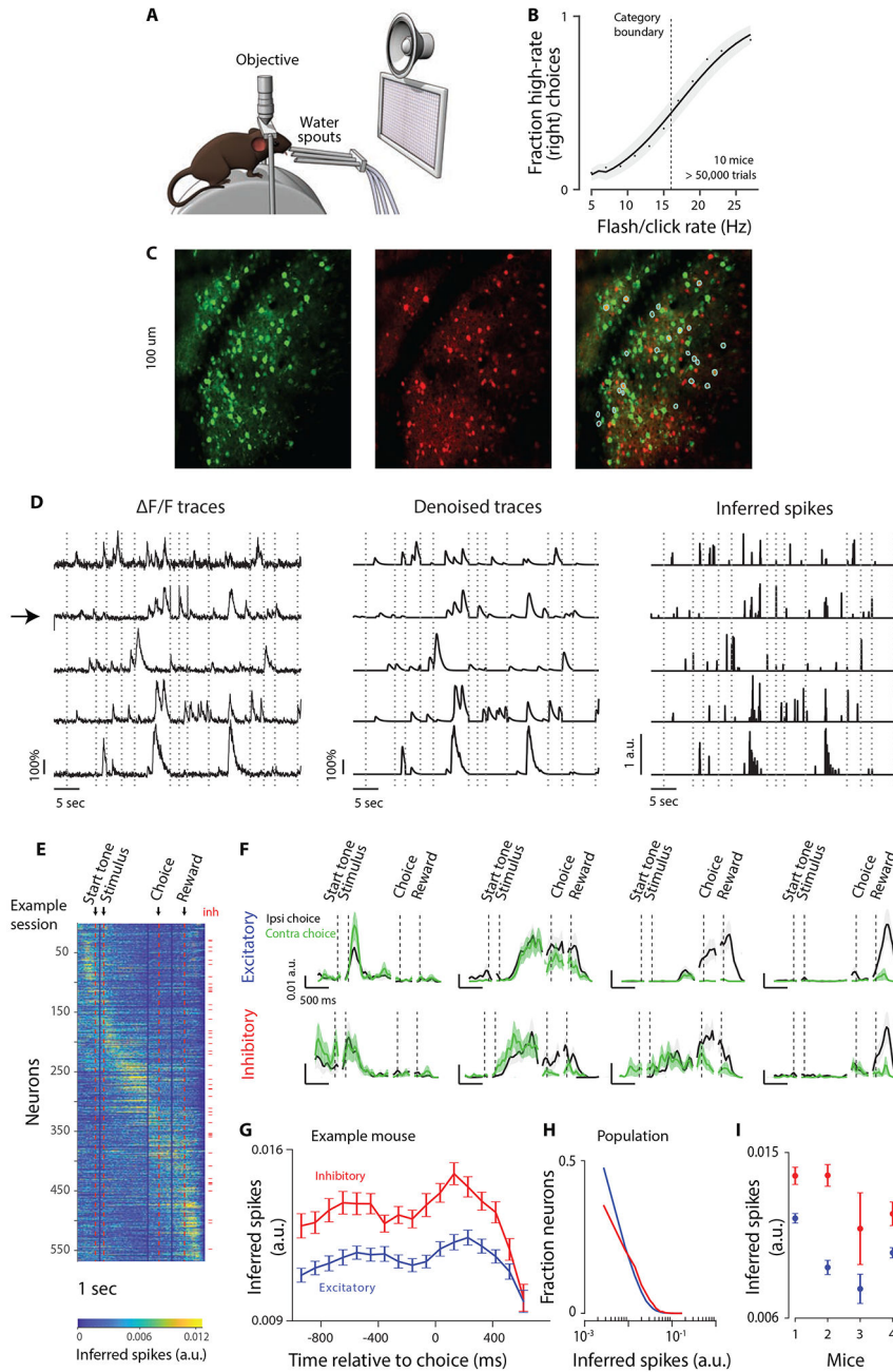
Figure 1. Simultaneous imaging of inhibitory and excitatory populations during decision-making.
