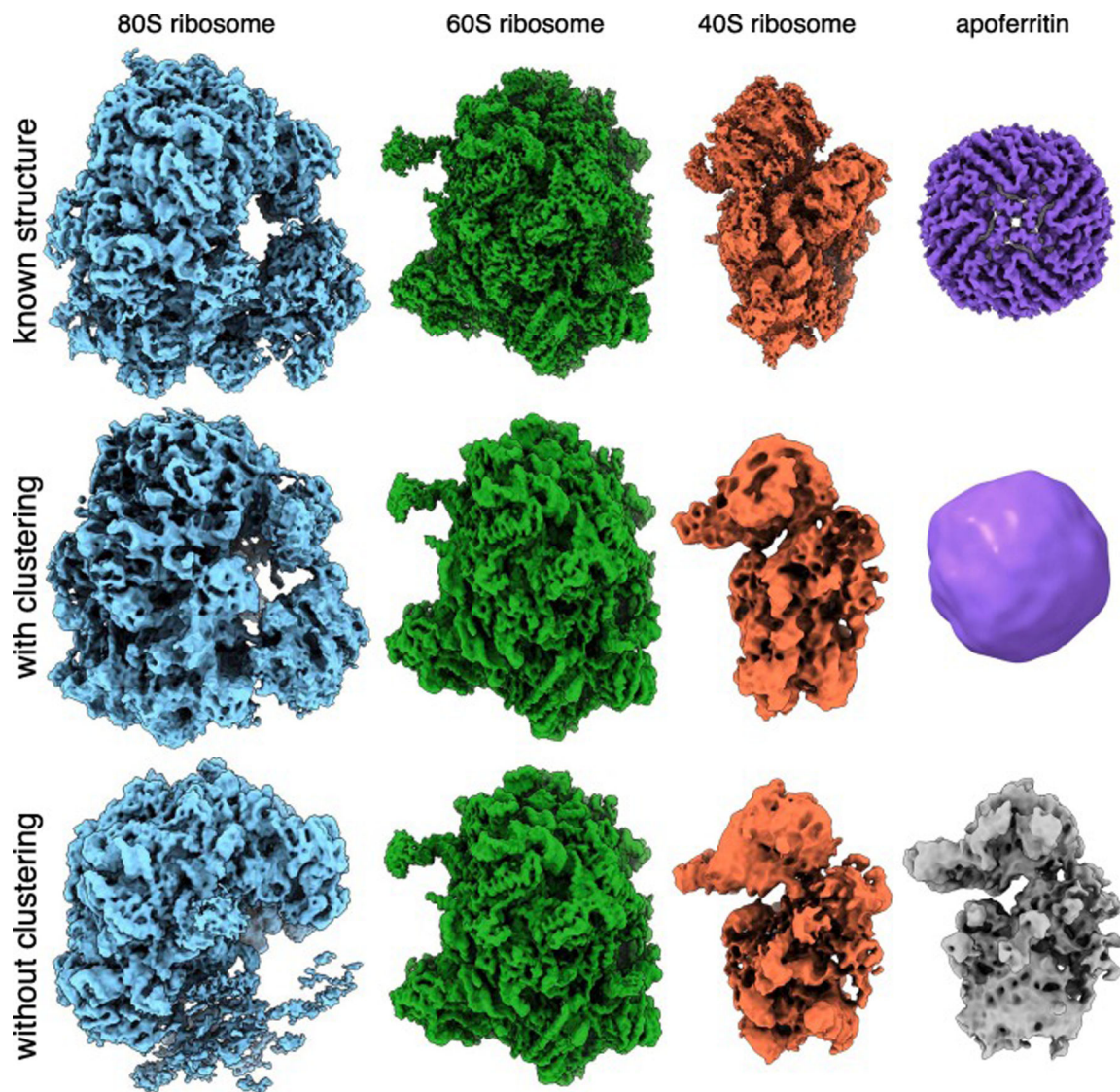
Figure 5. Ab initio structures from an experimental mixture
