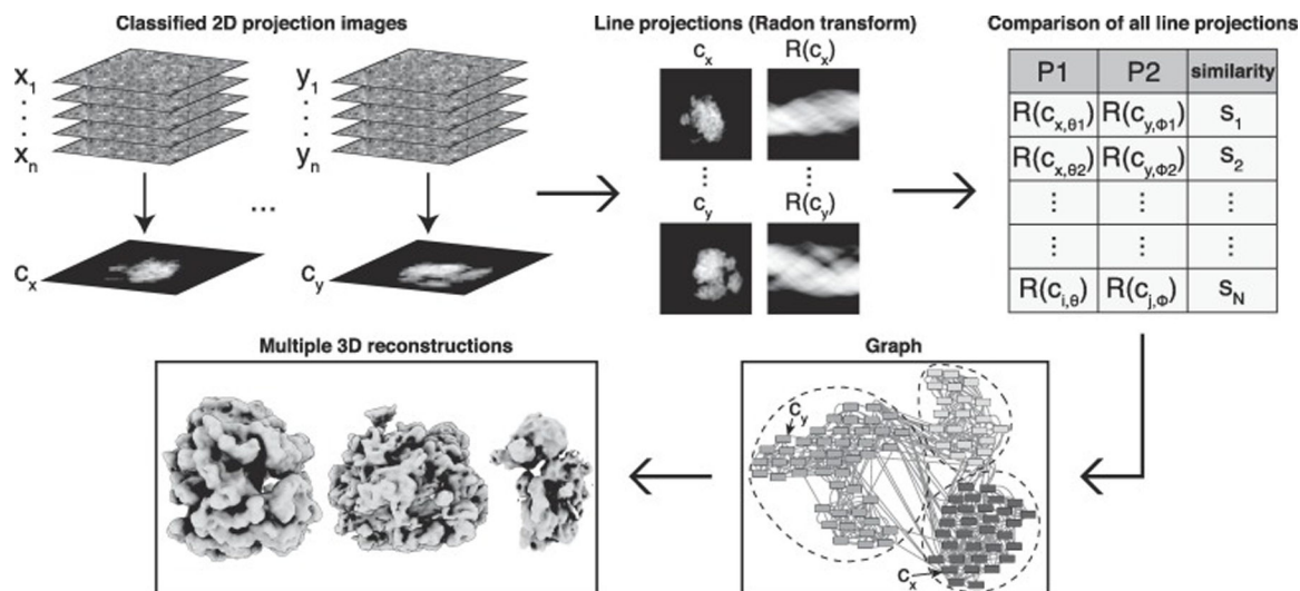
Figure 1. Computational pipeline for SLICEM
