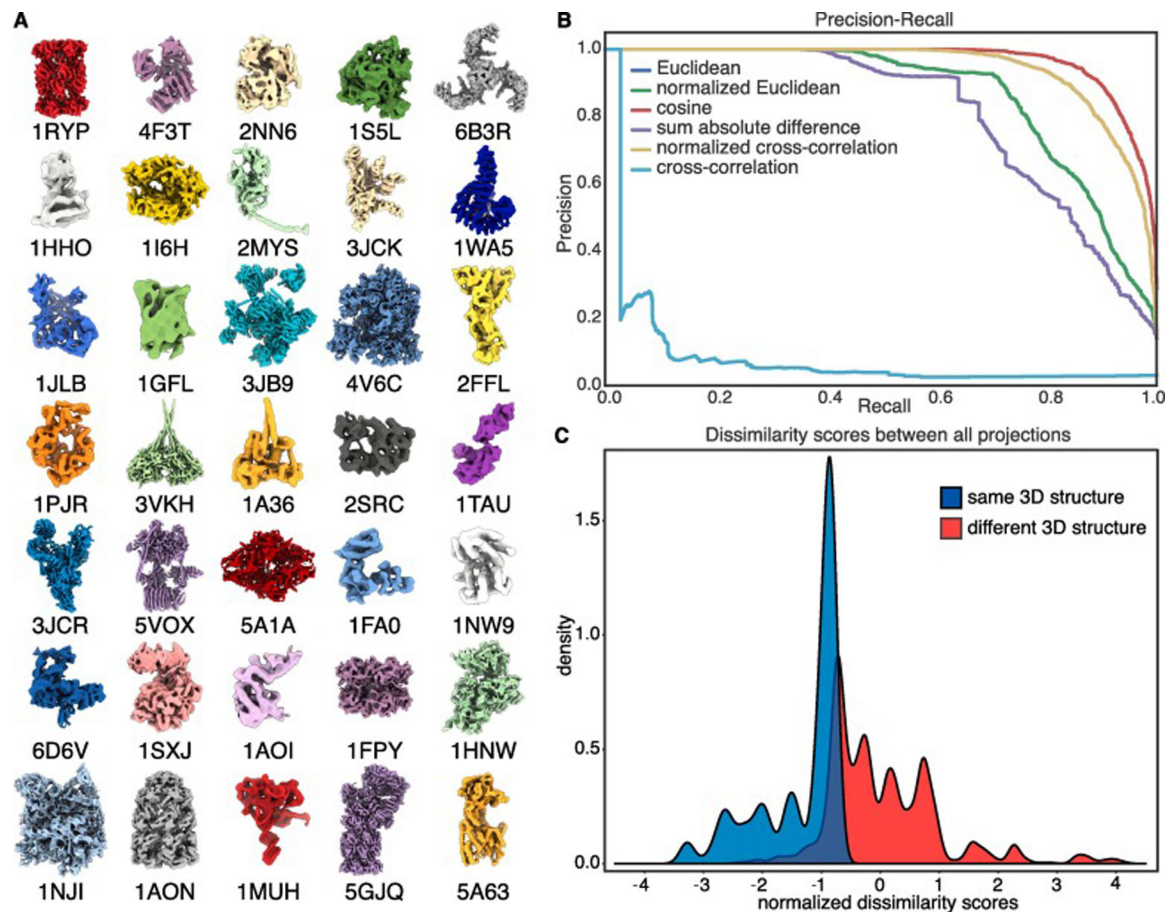
Figure 2. Separating mixtures of synthetic 2D reprojections
