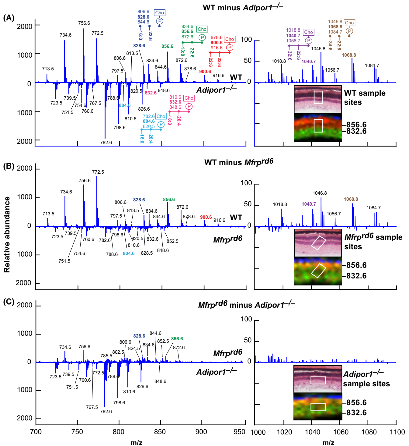
FIGURE 3 Differential MALDI spectra reveal compensatory PCs generated in Adipor1 -/- and the Mfrprd6 retina. Difference spectra show relative abundances detected by MALDI IMS. A, Molecules more abundant in WT retina vs Adipor1 -/- retina are presented in the upper part of the graph, while molecules more abundant in the Adipor1 -/- retina are displayed at the bottom. 22:6- and/or VLC-PUFA-containing PCs are much more abundant in WT while 20:4-containing PCs are increased in the mutant retina. The regions from which the spectra are extracted are shown in the insets H and E (top) and MALDI (bottom), showing PC40:6 ( m/z = 856.6 , red) and PC38:4 ( m/z = 832.6 , green). The identification of the mass numbers is shown in Supplemental Table 3. B, The difference spectra of Mfrprd6 to WT. (C) The difference spectra of Adipor1 -/- to Mfrprd6 . Inset images show that in both mutants, the PRC layers contain both PCs 40:6 and 38:4 (yellow) while WT has clear separation of the two PCs species between PRC layer and inner retina layer
