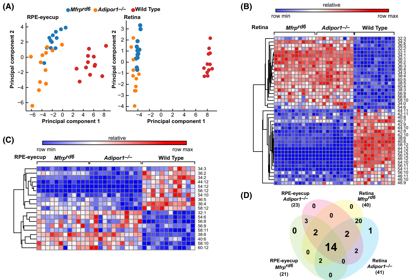
FIGURE 6 PCs containing VLC-PUFAs in Adipor1 -/- and Mfrprd6 eyes are greatly reduced. A, Principal component analysis of targeted PCs illustrates tissue-specific lipid profiles in mutants and WT mice (n = 12). B, C, Hierarchical clustering of significantly differentially occurring PC species (ANOVA one-way) in Adipor1 -/- and Mfrprd6 retinas and RPE-eyecups compared to WT ( P \leq .05 , absolute value fold-change \geq 1.5 ) suggests compensatory PC dynamics. D, Venn diagram illustrates overlap of differentially occurring PCs across strains and tissues
