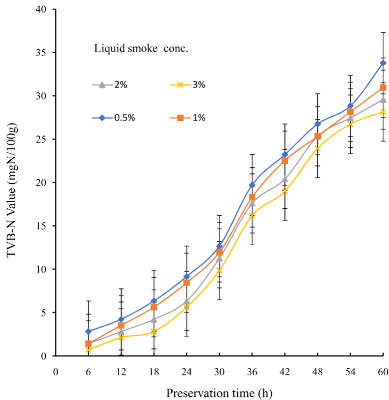
Figure 2. Association between preservation time, liquid smoke concentration and TVB-N value (liquid smoke was produced at 380°C).
