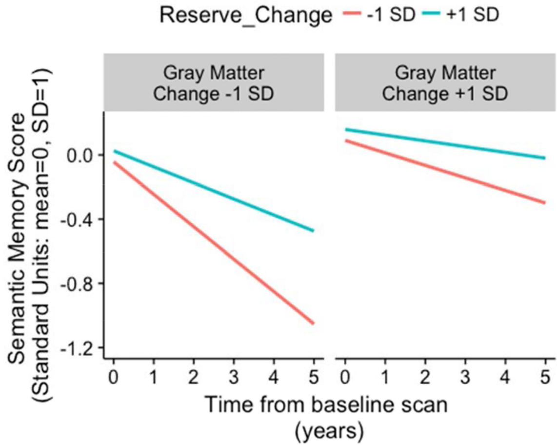
Figure 4. Expected 5-y longitudinal cognitive trajectory of semantic memory for specific reserve change levels (-1 and +1 SD) and specific cortical gray matter atrophy rates (-1 and +1 SD).
