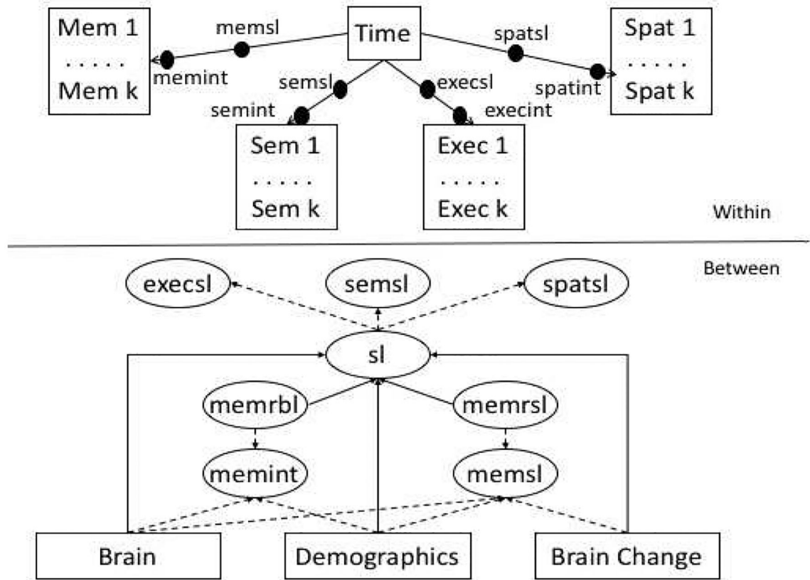
Figure 1. Longitudinal Reserve Model.
