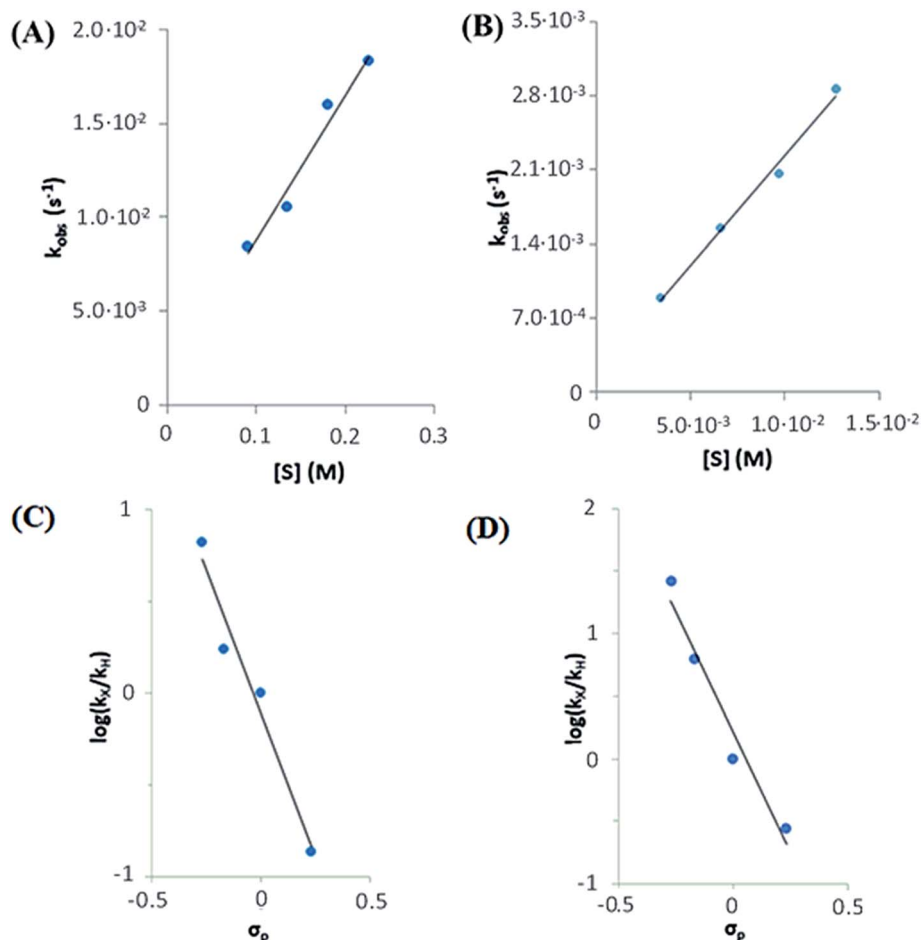
Fig. 9 Top: rate dependence on substrate concentration of reactions of (A) 1^{(IV)}=NTs (left) with Me^O PhSMe substrate (denoted as [S]) and (B) 2^{(IV)}=NTs with Me^O PhSMe substrate (right) at 293 K. Bottom: Hammett plot representing \log(k_x/k_H) against Hammett parameter ( \sigma_p ) for the reactions of (C) 1^{(IV)}=NTs (left) and (D) 2^{(IV)}=NTs (right) with p -X-thioanisoles in acetonitrile at 293 K. k_x values correspond to the second order rate constants obtained by measuring k_{obs} values at different p -X-thioanisole concentrations.
