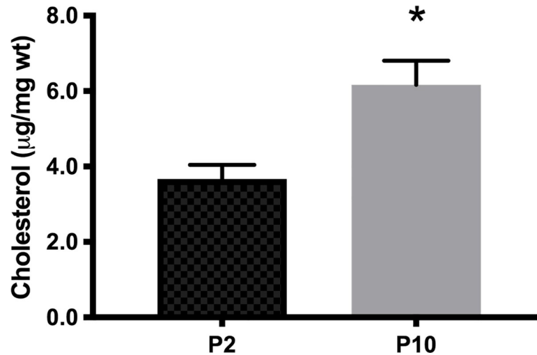
Fig 4. Cholesterol concentrations in whole brains of C57BL6 mice at postnatal days 2 (P2) and 10 (P10). Data are expressed as µg of cholesterol/mg of wet tissue (µg/mg wt). Bars represent mean ± SEM (n = 3); * p < 0.05, Student's t-test.
