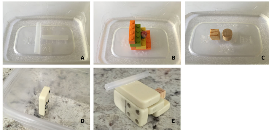
Fig. 1 Puzzle phantoms used during Phase 1. a Rotation puzzle. b Depth puzzle. c Sliding puzzle. d Tilting puzzle. e Assessment phantom
