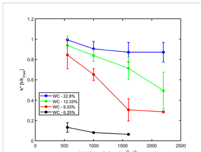
FIGURE 4 | Effect of light intensity on normalized soil-plant conductance k^* = k/k_{max} (where k_{max} is the soil-plant conductance in the wettest soil and lowest light intensity) at varying soil water contents (WC). Relative soil-plant conductance k^* decreased with increasing light intensity due to higher transpiration rates and with decreasing soil water contents due to the decreasing soil hydraulic conductivity.
