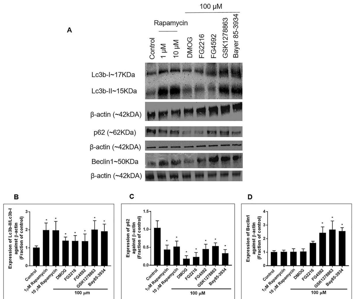
Figure 3. Immunoblot analysis of the protein expression of Lc3b-II, Lc3b-I, p62 and Beclin1 in PC12 cells treated with the indicated PHD inhibitors (100 μM) and rapamycin (1 & 10 μM) for 24 hours in normoxia. (A) Representative immunoblots of Lc3b-II, Lc3b-I, p62 and Beclin1 were shown alongside β-actin; (B) Normalised Lc3b-II/Lc3b-I ratio measured after 24 hours exposure to the indicated PHD inhibitors and rapamycin in normoxia (n = 3). Significant increase in the Lc3b-II/Lc3b-I ratio was seen with rapamycin (1 & 10 μM) and 100 μM of DMOG, FG2216, FG4592, GSK1278863 and Bay85-3934. GSK1278863 and Bay85-3934 had a similar effect on the Lc3b-II/Lc3b-I ratio as Rapamycin; (C) Expression of p62 measured after 24 hours exposure to the indicated PHD inhibitors and rapamycin in normoxia (n = 3). Significant reduction in p62 expression in comparison to vehicle (1% DMSO)-treated cells was seen with rapamycin (1 & 10 μM) and 100 μM of DMOG, FG2216, FG4592, GSK1278863 and Bay85-3934 treated cells; (D) Expression of Beclin1 measured after 24 hours exposure to the indicated PHD inhibitors and rapamycin in normoxia (n = 3). Significant upregulation of Beclin1 expression in comparison to vehicle (1% DMSO)-treated cells was seen in 100 μM of DMOG, FG2216, FG4592, GSK1278863 and Bay85-3934 treated cells, but was not in the Rapamycin treated cells. Data were expressed as mean ± S.D. *Indicated P < 0.05 against 1% DMSO treatment (Two-way ANOVA, Tukey's post-hoc analysis).
