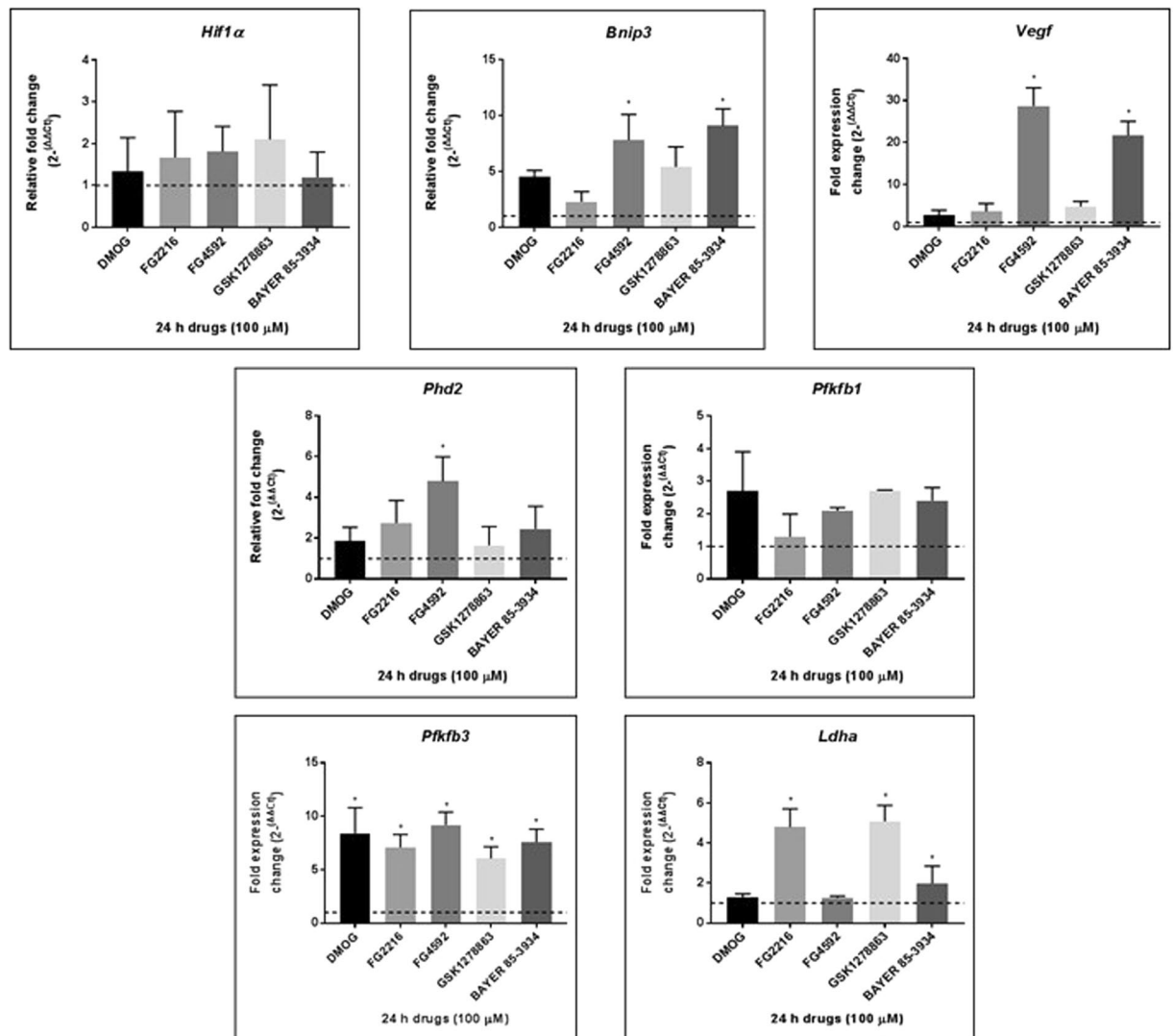
Figure 5. Effects of HIF PHD inhibitors on hypoxia gene expression. Expression of hypoxia genes, HIF1α , Bnip3 , Phd2 , Vegf , Pfkfb1 , Pfkfb3 , Ldha , after treatment with 100 \mu M PHD inhibitors in normoxia for 24 hours were normalised to \beta -actin levels. Significant upregulation of Bnip3 and Vegf was seen with FG4592 and Bay85-3934. Phd2 was significant upregulated by FG4592. Pfkfb3 was significantly upregulated by DMOG, FG2216, FG492, GSK1278863, and Bay85-3934. Ldha was significantly upregulated by FG2216, GSK1278863 and Bay85-3934. HIF1α was not changed by any of the HIF PHD inhibitors. Each data point represented the mean and standard deviation of the relative fold change with respect to 1% DMSO-treated sample normalised to reference gene \beta -actin level. The dotted line represented basal gene expression. Statistical significance was indicated as * P < 0.05 (Two-way ANOVA, Tukey's post-hoc analysis).
