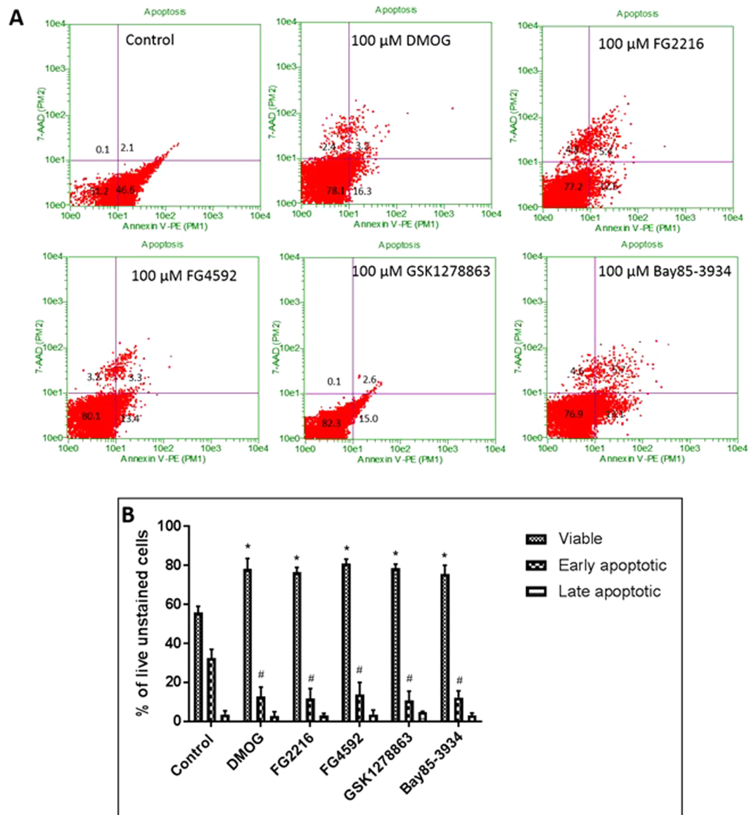
Figure 7. Annexin-V/7-AAD FACS analysis of PC12 cells preconditioned with the HIF PHD inhibitors followed by 24 hours re-oxygenation and 6 hours OGD. PC12 cells were exposed to PHD inhibitors (100 μM) for 24 hours in normoxia (21% O 2 ), followed by 24 hours re-oxygenation (21% O 2 ) and subsequent 6 hours OGD treatment (0.3% O 2 ). (A) Representative dot plots of Annexin-V/7-AAD FACS analysis of cells with the PHD inhibitor pre-treatment and 24 hours re-oxygenation followed by 6 hours OGD. Cells in the lower left quadrant represent viable cells, cells in the lower right quadrant represent early apoptosis and cells in upper right quadrant represent late apoptosis/necrosis; (B) The group data (n = 3) representing % of viable, early and late apoptotic cells. Significant reductions in the fractions of early apoptotic cells were seen in cells preconditioned with 100 μM of DMOG, FG2216, FG4592, GSK1278863 and Bay 85-3934 in comparison to 1% DMSO-treated cells following 24 hours re-oxygenation and 6 hours OGD. Data were expressed as mean ± S.D. *Indicated significance of viable cells P < 0.05 against 1% DMSO. #Indicated significance of apoptotic cells P < 0.05 against 1% DMSO (Two-way ANOVA, Tukey's post-hoc analysis).
