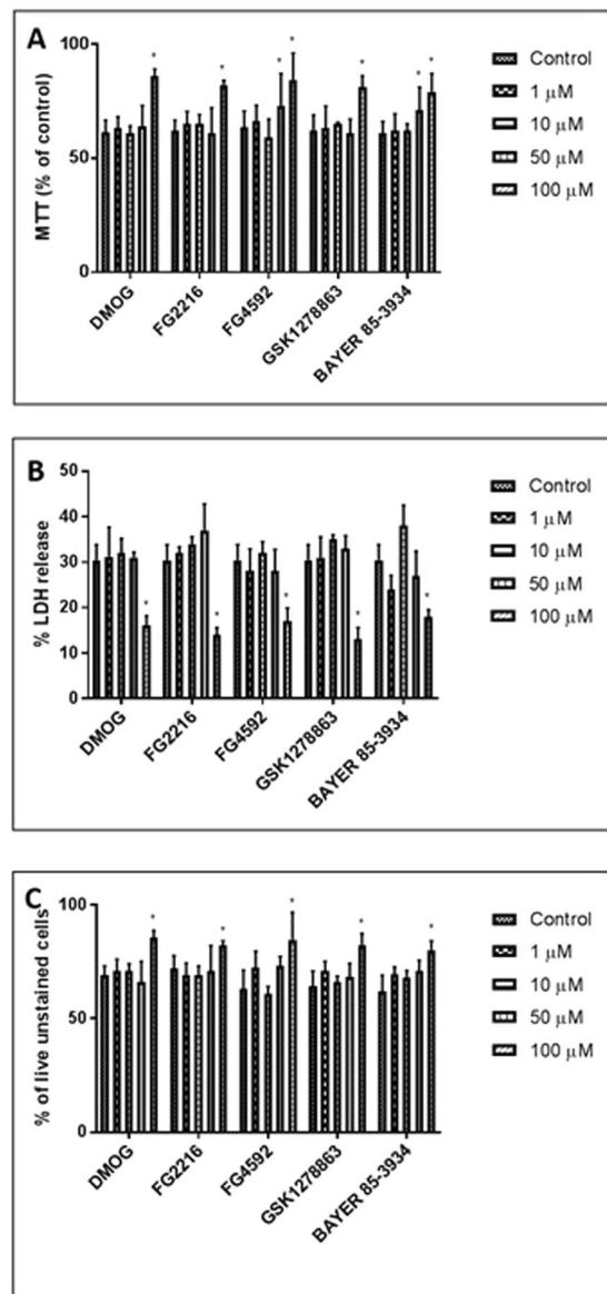
Figure 6. The effect of preconditioning with HIF-PHD inhibitors followed by 24 hours re-oxygenation and 6 hours OGD on PC12 cells. PC12 cells were exposed to the PHD inhibitors (1, 10, 50 and 100 \mu M) for 24 hours in normoxia (21% O_2 ) followed by 24 hours re-oxygenation (21% O_2 ) and subsequent 6 hours OGD insult (0.3% O_2 ). (A) MTT assay ( n = 3 ) showed greater mitochondrial activity after 6 hours OGD in cells preconditioned with 100 \mu M of DMOG, FG2216, or GSK1278863 and 50 & 100 \mu M of FG4592 or Bay 85-3934 compared to 1% DMSO pretreatment; (B) LDH assays ( n = 3 ) revealed reduced LDH release in cells preconditioned with 100 \mu M of DMOG, FG2216, FG4592, GSK1278863, or Bay 85-3934 prior to 6 hours OGD compared to 1% DMSO pretreatment; (C) Trypan blue exclusion assays ( n = 3 ) reveal increased live (unstained) cells in cells preconditioned with 100 \mu M of DMOG, FG2216, FG4592, GSK1278863, or Bay 85-3934 prior to 6 hours OGD compared to 1% DMSO pretreatment. Data were expressed as mean \pm S.D. *Indicated P < 0.05 against 1% DMSO (Two-way ANOVA, Tukey's post-hoc analysis).
