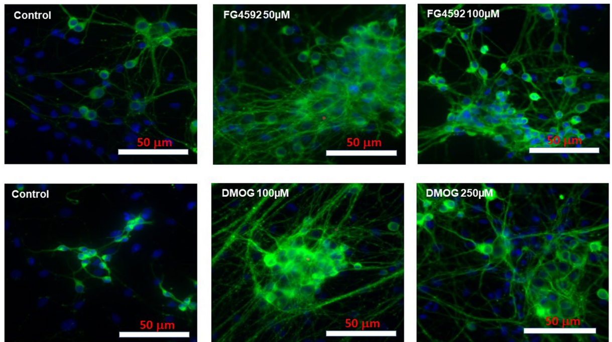
Figure 13. Representative double merged (FITC labelled neuron specific Tuj1 and DAPI stained nuclei) immunofluorescence images of primary rat neurons preconditioning with FG4592 and DMOG followed by 6 hours OGD. FG4592 (50, 100 \mu M) and DMOG (100, 250 \mu M) preconditioned neurons displayed longer and more neurites than those pretreated with 1% DMSO.
