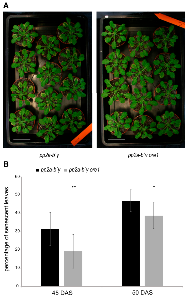
Figure 6. Senescence progression in pp2a-b'γ and pp2a-b'γ ore1 leaves. A, Photographs depicting leaf yellowing in pp2ab'γ and pp2ab'γ ore1 leaves, 45 DAS. Scale bars = 5 cm. B, Quantification of senescence progression in pp2ab'γ and pp2ab'γ ore1 leaves shown in (A), expressed as percentage of the number of leaves showing any visual symptoms of yellowing and cell death from all leaves of the plant. Data are means ( n_{\text{plants}} = 12 \pm \text{SD} ). Statistically significant differences to pp2ab'γ are indicated by asterisks. Student's t test, ** P < 0.005 ; * P < 0.01 .
