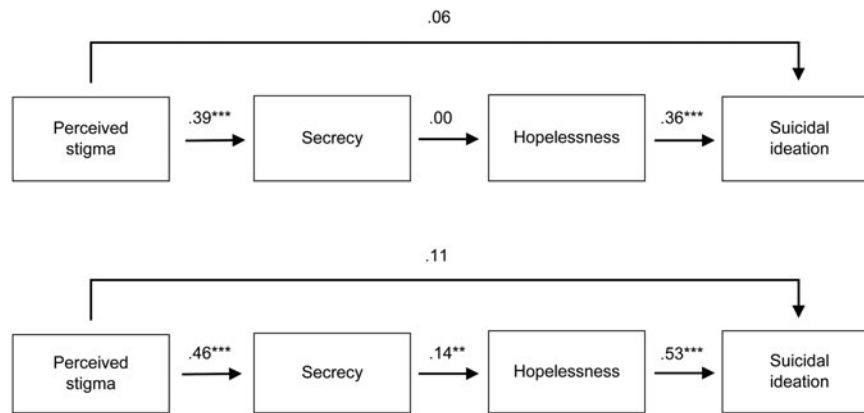
Fig. 1. Results obtained from the path analyses, testing the three-path mediation effect of secrecy and hopelessness among unlabelled persons (upper path diagram, N = 252 , R^2 = 0.19 ) and individuals labelled by lifetime mental health service use (lower path diagram, N = 429 , R^2 = 0.26 ). ** p < 0.01 , *** p < 0.001 .
