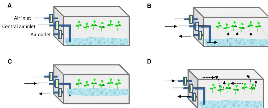
FIGURE 3 Plantform™ bioreactor. (A) The pump is off and the liquid medium is in the lower compartment, separate from the explants, (B) the pump impules air through the central inlet filter, (C) the overpressure moves the medium up and cause immersion of the explants, as well as air expulsion through the outlet filter. When the pump is off, the medium goes down by gravity, and (D) additional aerations: the pump impules air through any of the lateral inlet filters. The air circulates through the chamber containing the explants, but does not cause translocation of the medium
