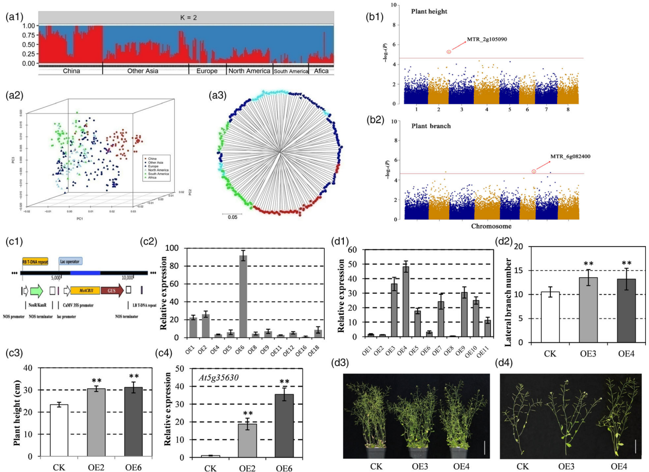
Figure 1 (a) Structure (a1), principal coordinate analysis (a2) and NJ tree (a3) of the alfalfa association panel using the marker data generated by GBS. (b) Manhattan plot showing significant alfalfa locus associated with plant height (b1), and plant branching (b2). Negative \log_{10}(P) values from a genome-wide scan are plotted against position on each of eight chromosomes. (c) Functional characterization of MsACR11 as an ACR-domain protein in Arabidopsis thaliana . (c1) Schematic showing the transfer DNA of the vector. (c2) expression analysis of MSACR11 in A. thaliana overexpression lines by qRT-PCR. Total RNA was extracted from 3-week-old A. thaliana transgenic lines. The data are shown as the means \pm SD of three biological replicates. (c3) the plant height of WT and transgenic A. thaliana plants. (c4) the transcription level of AtGLN2 ( At5g35630 ) in transgenic lines and WT plants (data are the means \pm SD of three biological replicates). (d) Functional characterization of MsPB1 in A. thaliana . (d1) the expression analysis of MsPB1 in A. thaliana transgenic lines by qRT-PCR. Total RNA was extracted from 3-week-old A. thaliana transgenic lines (data are the means \pm SD of the biological replicates). (d2) the plant branch number of transgenic A. thaliana and WT plants (means \pm SD, n = 6 ). (d3) phenotypes of plants of control (wild type col-0) and transgenic lines. (d4) phenotypes of lateral branches in control and transgenic plants. CK, Control (Col-0); OE, Overexpression. Bars = 5 cm in d3 and d4. *** in c3, c4 and d2 indicated P < 0.01 .
