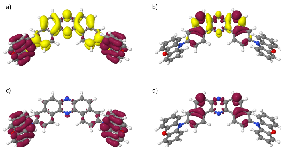
Figure 4. Difference densities (lisovaluel = 0.001) of (a) the S_1(\text{CT}) state and (b) the T_3(\pi\pi^*) state of POZ-DBPHZ. A loss of electron density with respect to the ground state is colored red, and a gain yellow. For the sake of clarity, the negative parts of the corresponding difference densities are shown in panels c and d, respectively.
