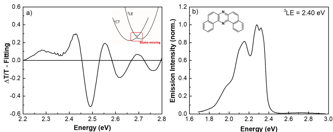
Figure 3. (a) Difference between the raw and fitted EA spectrum of POZ-DBPHZ in a zeonex matrix. The inset shows a theoretical diagram of the state mixing between 1 CT and 3 LE that results in the transfer of oscillator strength to the 3 LE state, thus allowing the state to be probed by EA measurements. (b) Normalized phosphorescence spectrum of DBPHZ (molecular structure shown in the inset) obtained with time-resolved measurements in a blend of 1% (w:w) DBPHZ in zeonex and a time delay above 25 ms. Onset measurement gives a state energy of 2.40 ± 0.02 eV.
