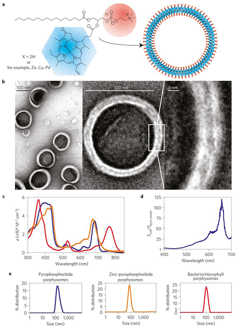
Figure 5. (a) A typical scheme for porphyrinsome, containing porphyrin and long-chain lipid. The phospholipid headgroup (red) and porphyrin (blue) are highlighted in the subunit (left) and assembled nanovesicle (right). (b), Electron micrographs of negatively stained porphyrinsomes (5% PEG-lipid, 95% pyropheophorbide-lipid). (c), Absorbance of the porphyrin-lipid subunits added in porphyrinsomes formed from pyropheophorbide (blue), zinc-pyropheophorbide (orange) and bacteriochlorophyll (red) in PBS. (d), Resonance light scattering spectra ratio between gold nanorods and pyropheophorbide porphyrinsomes. Nanorod and porphyrinsome concentration was adjusted to have equal optical density at 680
