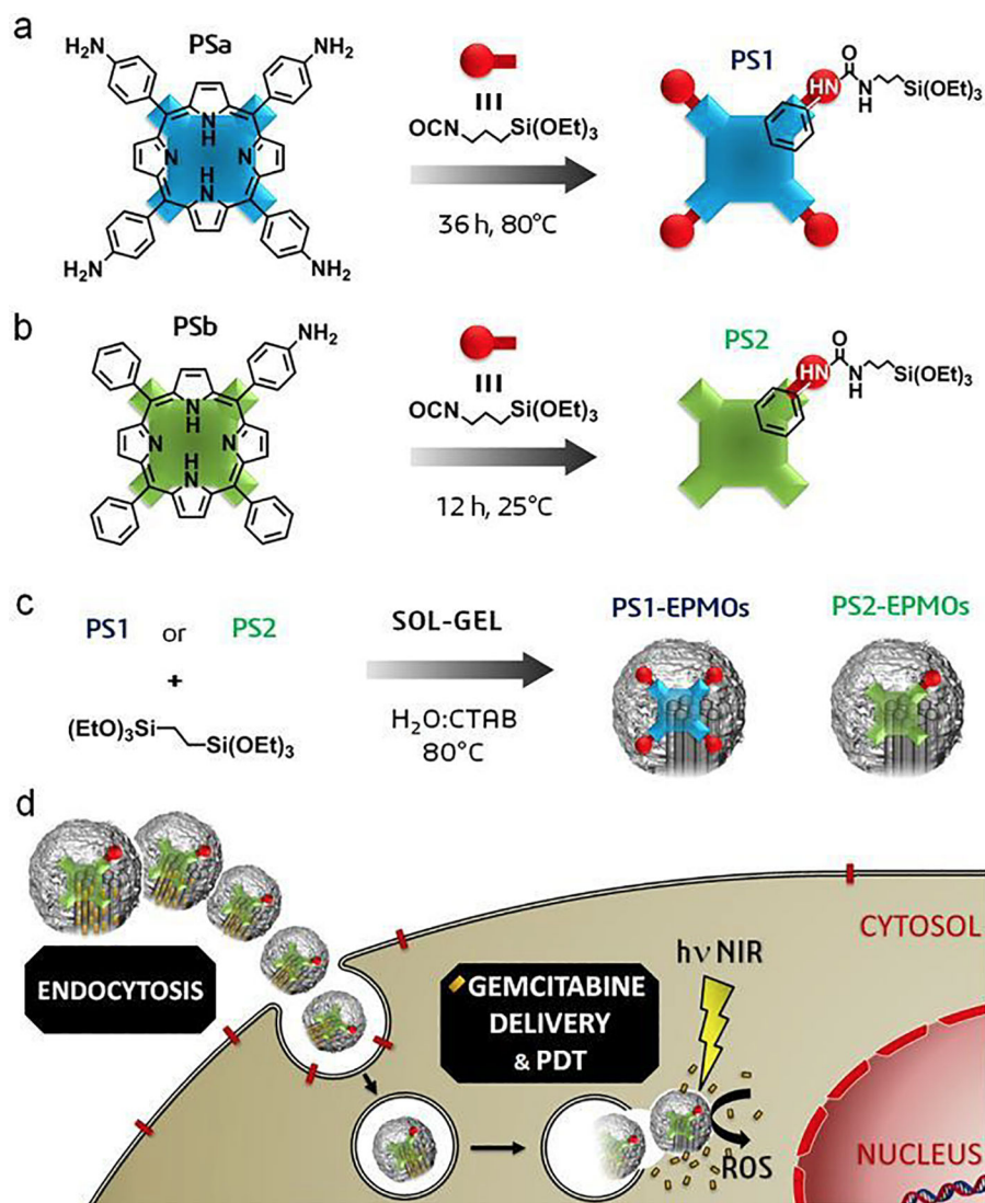
Figure 3. PS1, PS2 and their photosensitizer precursors Silylation (a and b). ethanephotosensitizer via PMO nanoparticles production by Sol-gel (c). Functions of PMO nanoparticles for drug delivery and photodynamic therapy (synergistic manner) (d) [35].
