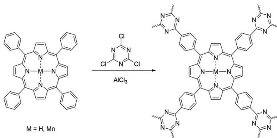
Figure 7. Schematic demonstration of the PCTF and PCTF-Mn producing [146]
