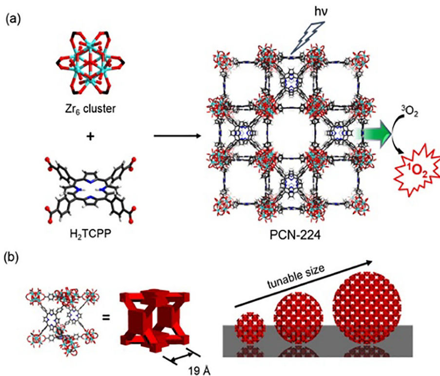
Figure 4. PCN-224 construction Image. (a) a cluster of Zr 6 with the open formula of (Zr 6 O 4 (OH) 4 (H 2 O) 6 (OH) 6 (COO) 6 ), tetratopic linker with the open formula of (tetrakis (4-carboxyphenyl) porphyrin with the open formula of (H 2 TCPP)), and image of PCN-224 as the 3D nanoporous framework. (b) A PCN-224 cubic unit and a schematic image of spherical PCN-224 NPs in cubic units structure form, potential to make various sizes [36].
