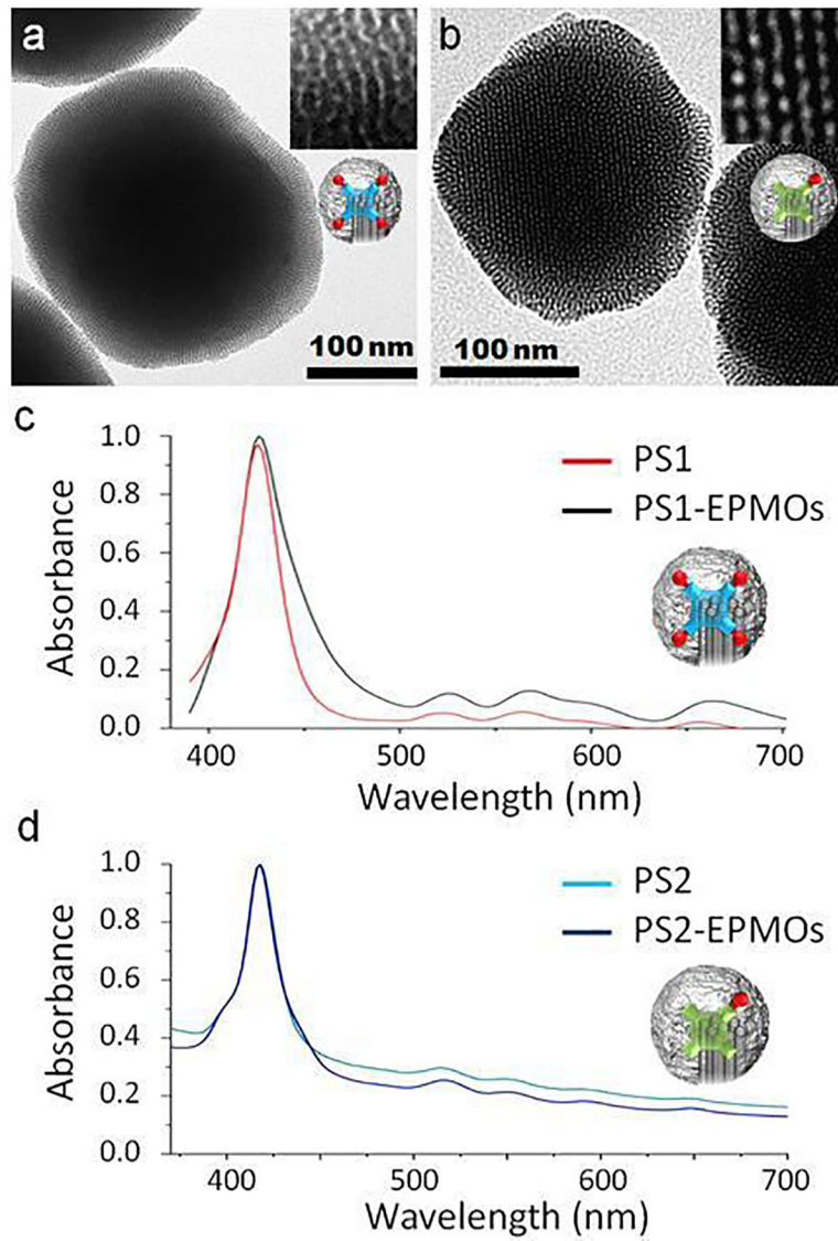
Figure 2. PS1-EPMO and PS2-EPMO nanoparticles and their HRTEM micrographs, respectively (a and b). Images exhibit usual mesoporosities. Photosensitizer precursors and their visible UV-spectrum via their NPs in EtOH (c and d) [35].
