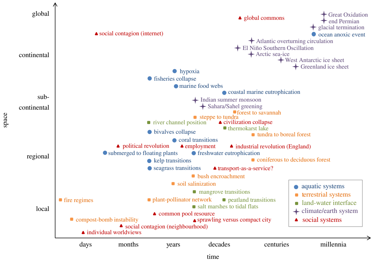
Figure 1. Examples of tipping points across system types and space and time scales—reworked from Biggs et al. [7] to include all climate tipping points [5] and additional examples discussed in the present text.
