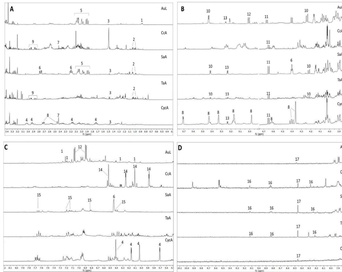
Figure 4. 1 H NMR extended spectral regions of AuL; CcA; SaA; TaA; CycA (from top to bottom). (A) region from δ 0.4 to 3.4; (B) from δ 3.4 to 5.4; (C) from δ 5.4 to 8.1; (D) from δ 7.8 to 10.00. Numbers indicate diagnostic signals of the most abundant metabolites: O-rhamnosyl flavonoid (1), valine (2), alanine (3), cynaropicrin (4), quinic acid (5), shikimic acid (6), succinic acid (7), malic acid (8), aspartic acid (9), sucrose (10), β-glucose (11), arbutin (12), α-glucose (13), sesquiterpene lactone-derivative (14), caffeic acid (15), trigonelline (16), formic acid (17). Spectra were measured in D 2 O-buffer (pH 6.0) using TMSF as standard, residual water signal has been removed.
