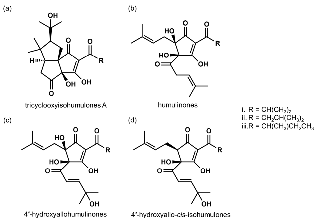
Figure 2. Chemical structures of representative MHBA components. (a) tricyclooxyisohumulones A; tricyclooxyisocohumulone A (i), tricyclooxyisohumulone A (ii), and tricyclooxyisoadhumulone A (iii). (b) humulinones; cohumulone (i), humulinone (ii), and adhumulinone (iii). (c) 4'-hydroxyallohumulinones; 4'-hydroxyallocohumulone (i), 4'-hydroxyallohumulinone (ii), and 4'-hydroxyalloadhumulinone (iii). (d) 4'-hydroxyallo- cis -isohumulones; 4'-hydroxyallo- cis -isocohumulone (i), 4'-hydroxyallo- cis -isohumulone (ii), 4'-hydroxyallo- cis -isoadhumulone (iii).
