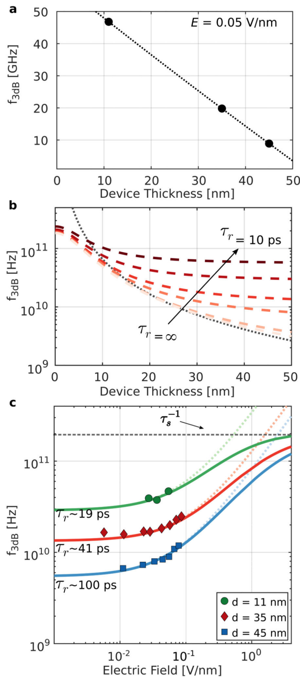
Fig. 5. Comparison of devices with different MoTe 2 thicknesses and under different bias conditions.
