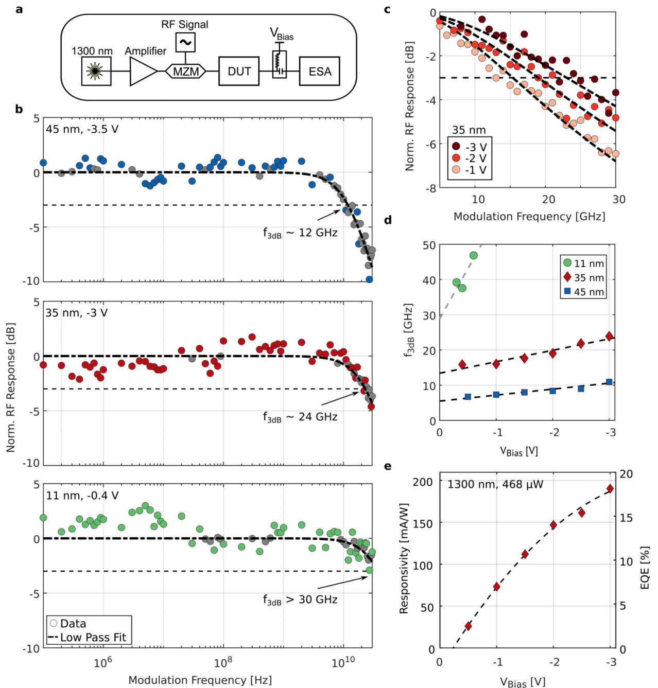
Fig. 4. Dynamic characterization of vertical photodetectors.
