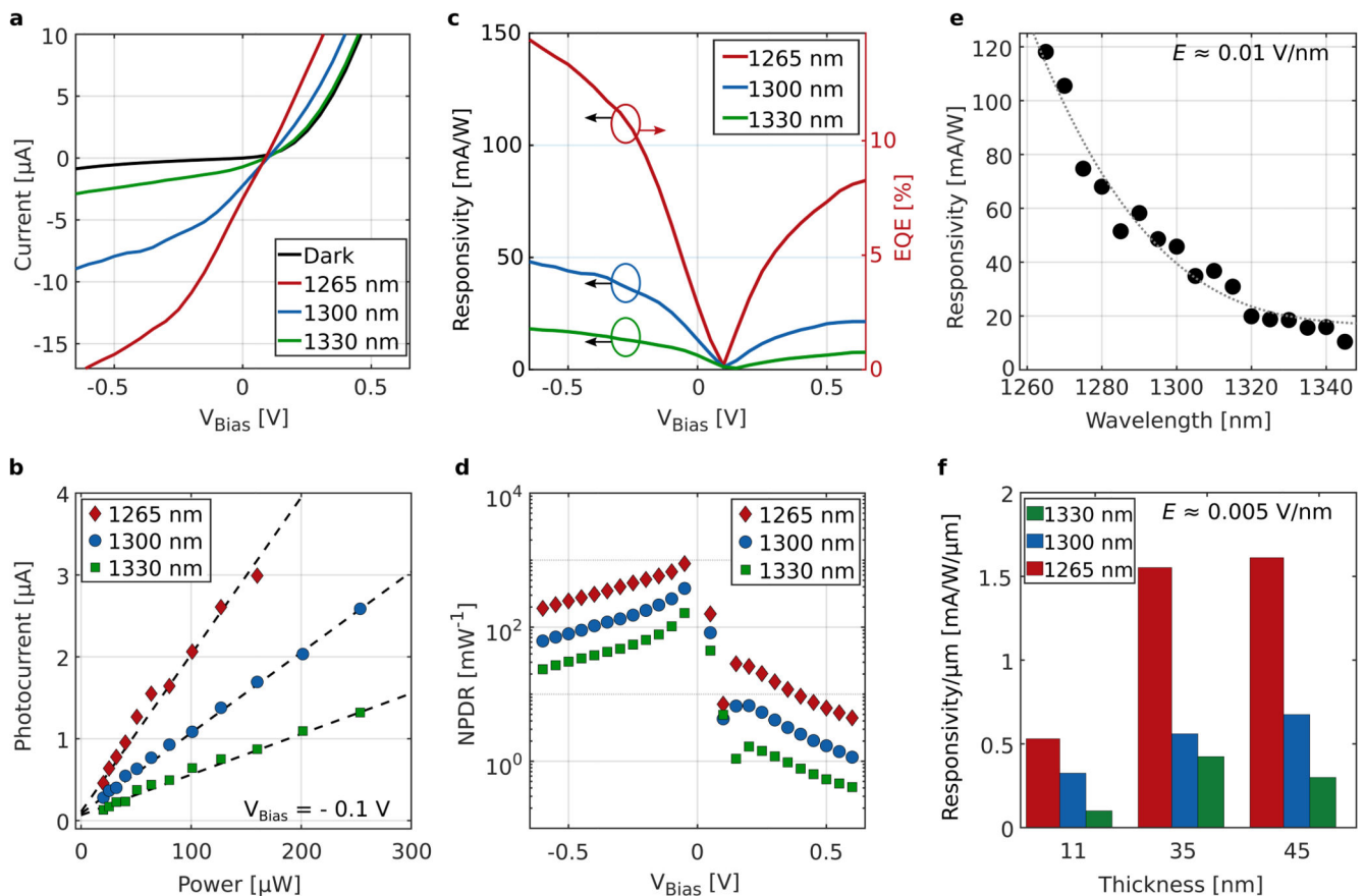
Fig. 3. Steady-state photoresponse of a waveguide photodetector featuring a MoTe 2 thickness of 45 nm.
