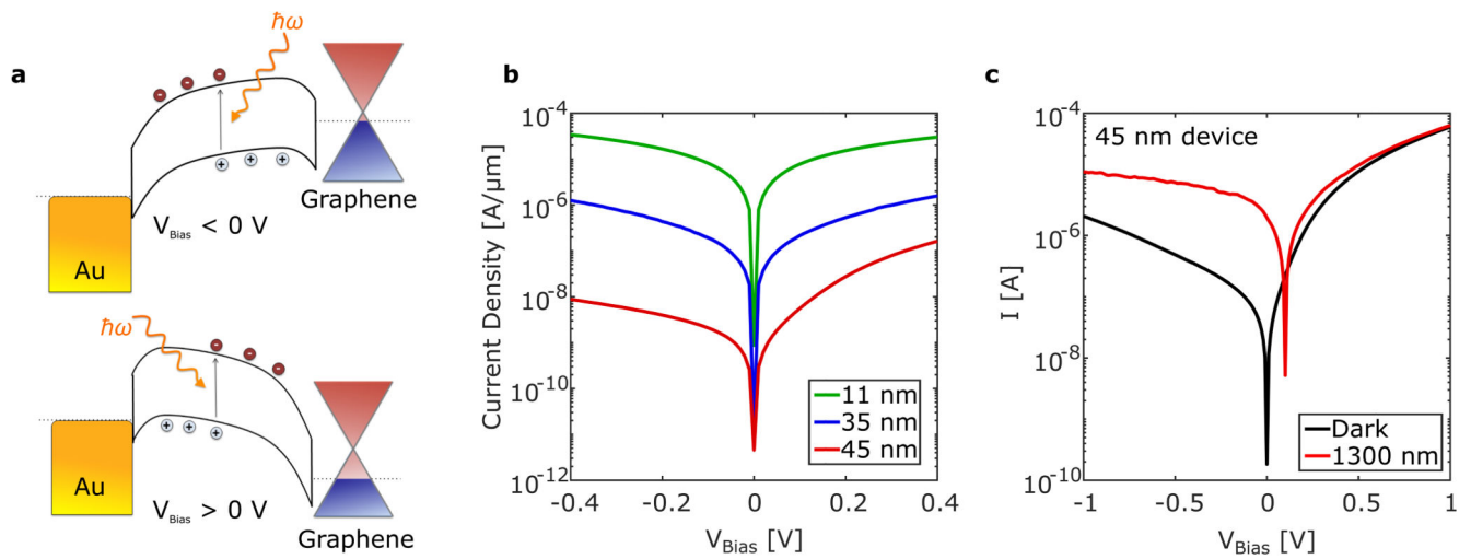
Fig. 2. Electrical Characteristics of the photodetector.
