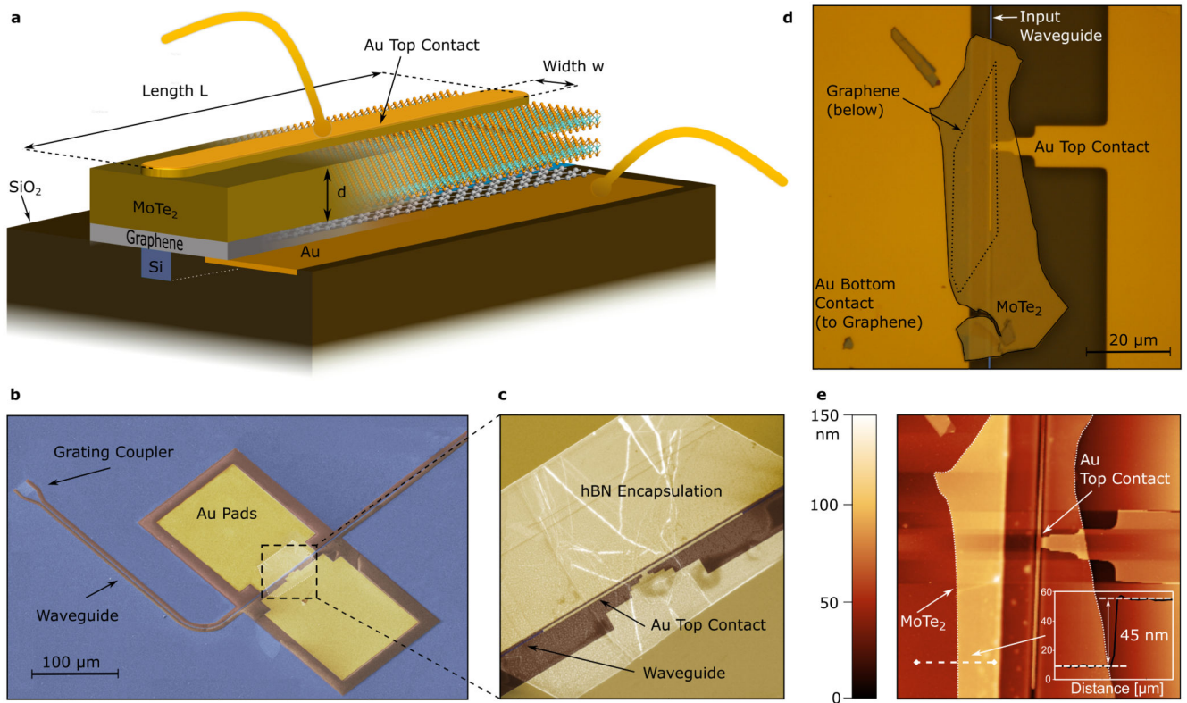
Fig. 1. Vertical MoTe 2 -graphene photodetector.
