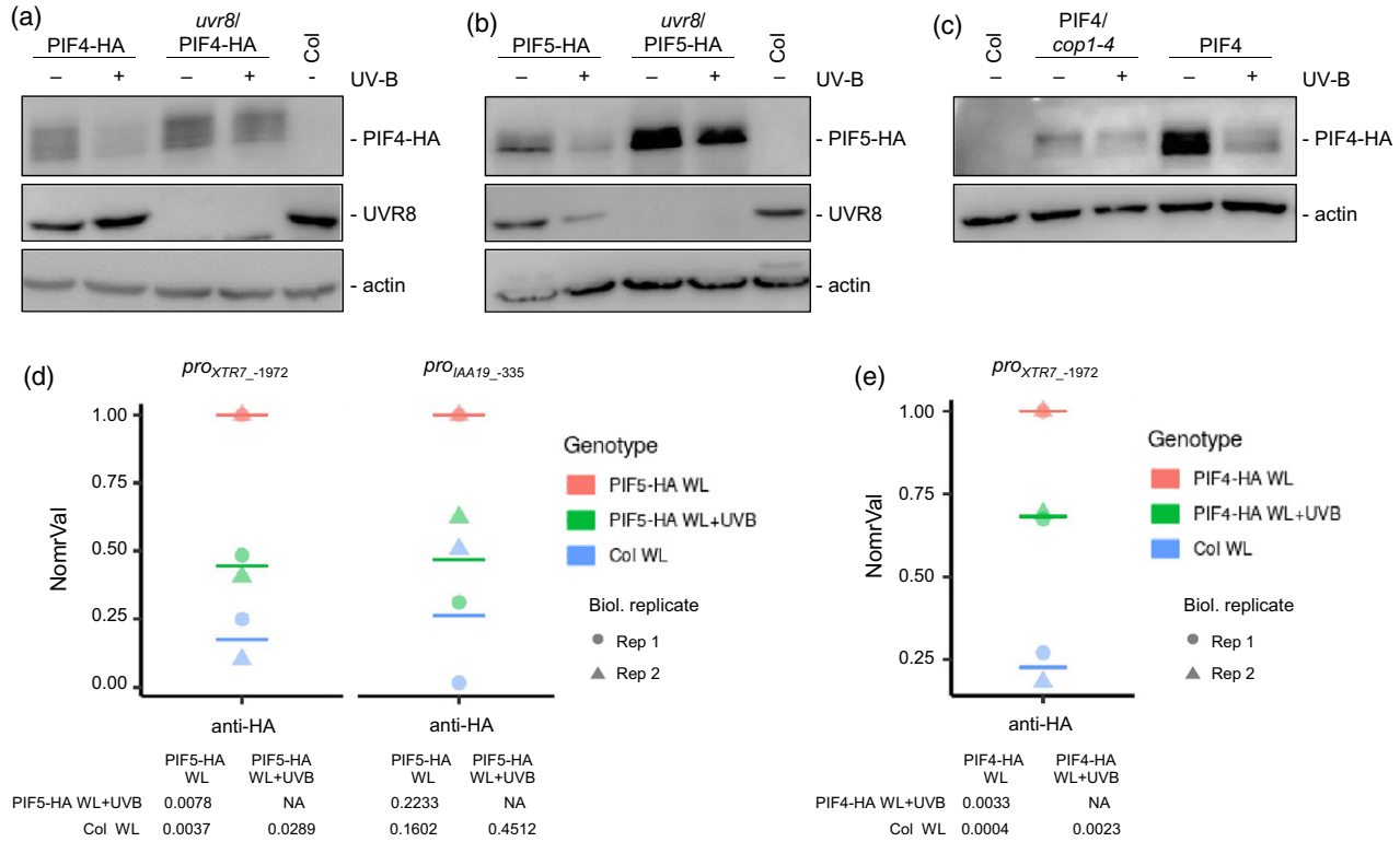
Figure 3. UVR8-mediated degradation of PIF4 and PIF5 is associated with reduced target promoter occupancy in response to UV-B. (a)–(c) Anti-hemagglutinin (HA) immunoblot analysis of HA-tagged proteins in 4-day-old seedlings grown under white light (–UV-B) or white light supplemented with a final 6 h of UV-B (+UV-B). The wild type (Col) is shown as a negative control. PIF4-HA protein levels (a) were analyzed in Col/ Pro PIF4 :PIF4-3×HA (PIF4-HA) and uvr8-6/Pro PIF4 :PIF4-3×HA ( uvr8/PIF4-HA ). PIF5-HA protein levels (b) were analyzed in Col/ Pro PIF5 :PIF5-3×HA (PIF5-HA) and uvr8-6/Pro PIF5 :PIF5-3×HA ( uvr8/PIF5-HA ). PIF4-HA protein levels (c) were analyzed in Col/ Pro PIF4 :PIF4-3×HA (PIF4-HA) and cop1-4/Pro PIF4 :PIF4-3×HA ( cop1-4/PIF4-HA ). Blots were reprobbed with anti-UVR8 (a,b), as well as anti-actin as loading control (a–c). (d) Chromatin immunoprecipitation (ChIP) of DNA associated with PIF5-HA. Chromatin immunoprecipitation-qPCR was performed for the XTR7 and IAA19 promoters and an intergenic region between the At4g26900 and At4g26910 genes using 5-day-old Col/ Pro PIF5 :PIF5-3×HA (PIF5-HA) seedlings either exposed to narrowband UV-B for 6 h (WL + UVB) or not (WL), and wild-type (Col; negative control) seedlings grown only under white light (WL). (e) Chromatin immunoprecipitation of DNA associated with PIF4-HA. Chromatin immunoprecipitation-qPCR was performed for the XTR7 promoter using 5-day-old Col/ Pro PIF4 :PIF4-3×HA (PIF4-HA) seedlings either exposed to narrowband UV-B for 6 h (WT + UVB) or not (WL) and wild-type (Col; negative control) seedlings grown only under white light (WL). In (d) and (e) the ChIP experiments were performed with an anti-HA antibody. The numbers of the analyzed DNA fragments ( pro XTR7-1972 , pro IAA19-335 ) indicate the positions of the base pair of the amplicon relative to the translation start site (referred to as position +1). The percentage of DNA associated with (d) PIF5-HA and (e) PIF4-HA relative to total input DNA of two independent biological replicates were normalized against the PIF5-HA WL and PIF4-HA WL sample, respectively (NormVal, PIF5-HA WL = 1 and PIF4-HA WL = 1). Means are represented as horizontal bars. P -values from pairwise t -tests using Holm’s correction for multiple tests are shown.
