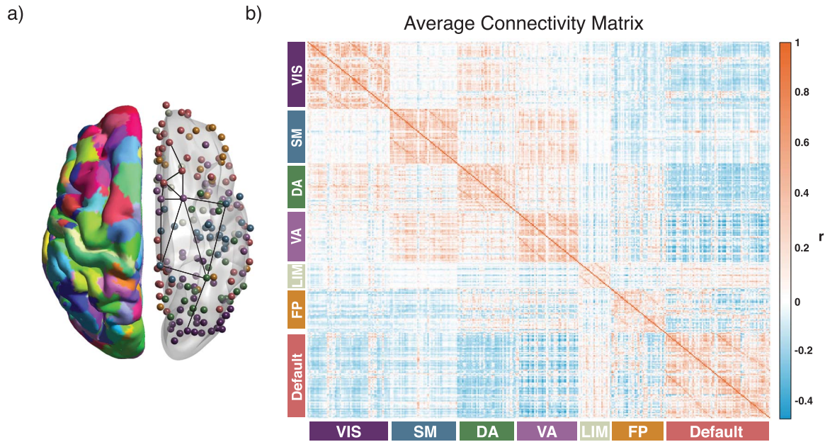
Figure 1. Schematic of approach. (a) A total of N = 360 regions of interest in a multimodal cortical parcellation (Glasser et al. 2016). From each region, we estimated the mean BOLD timeseries, and then we calculated the functional connectivity between any two regions using the Pearson correlation coefficient. For each subject, we collated all functional connectivity estimates into a single N \times N adjacency matrix. The left hemisphere depicts the parcellation, while the right hemisphere depicts regions represented as network nodes and colored by their association to putative cognitive systems (Yeo et al. 2011). (b) The average functional connectivity matrix across subjects, ordered by putative cognitive systems. VIS: visual; SM: somatomotor; DA: dorsal attention; VA: ventral attention; LIM: limbic; FP: frontoparietal.
