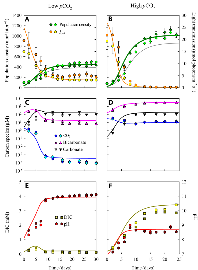
Fig. 4. Population density, inorganic carbon chemistry, and pH in chemostat experiments with Microcystis PCC 7806 at low and at high p\text{CO}_2 . Chemostat experiments were performed in duplicate, at low p\text{CO}_2 (left) and at high p\text{CO}_2 (right). (A and B) Microcystis population density ( n = 3 technical replicates per chemostat) and light intensity I_{\text{out}} transmitted through the chemostat ( n = 10 ). (C and D) Dissolved CO 2 , bicarbonate, and carbonate concentrations. (E and F) Dissolved inorganic carbon (DIC) and pH ( n = 3 technical replicates per chemostat). Symbols indicate experimental data of the duplicate chemostat experiments, error bars indicate SDs of technical replicates, and lines indicate model predictions. Error bars in (E) and (F) did not exceed the size of the symbols. For comparison, gray lines in (A) and (B) are model predictions for nonacclimated cells that either (A) grow at low p\text{CO}_2 but with carbon uptake kinetics acclimated to high p\text{CO}_2 or (B) grow at high p\text{CO}_2 but with carbon uptake kinetics acclimated low p\text{CO}_2 . Steady-state characteristics of the experiments are summarized in table S1, and parameter values of the model are listed in tables S4 and S5.
