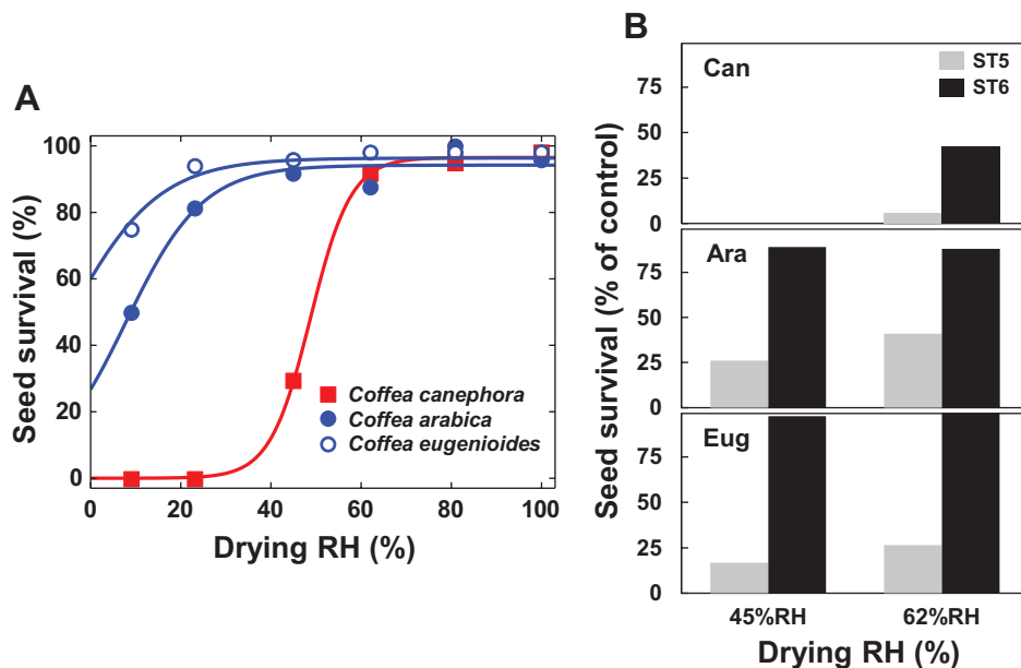
Fig. 1. Characterization of seed desiccation tolerance in the three coffee species, Coffea arabica , C. canephora , and C. eugenoides . (A) Survival rate of mature (stage 7) coffee seeds after equilibration drying at various relative humidity (RH) conditions. The curves correspond to the fitted patterns using the quantal response model described in Dussert et al. (1999). (B) Changes in viability (%) after equilibration drying at various RH conditions during seed development (stage 5–6).
