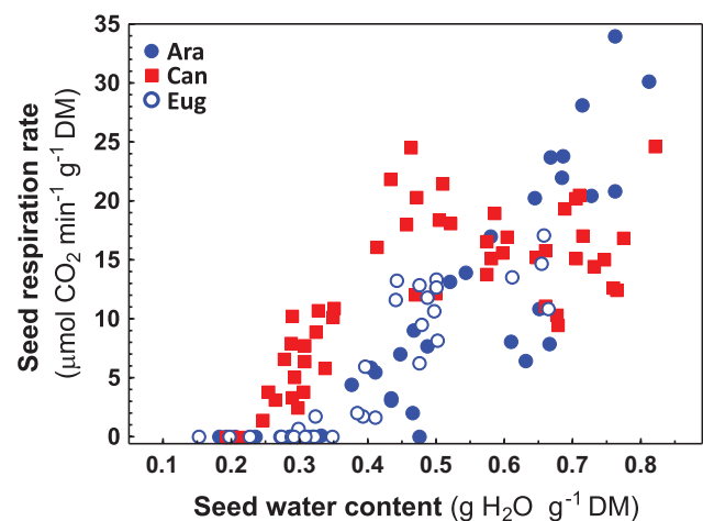
Fig. 7. Respiration rates, measured as release of CO 2 (µmol CO 2 min -1 g -1 DM) as a function of the hydration state (g H 2 O g -1 DM) of fresh mature seeds (ST7) of the three coffee species during equilibrium drying.
