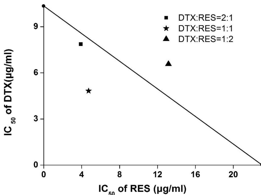
Fig. 2 – The isobologram of DTX and RES at different ratios. The straight line (additive line) connects the IC 50 values of DTX and RES when the drugs were used alone, and the points plotted on the isobolograms were based on the result of Table 1.
