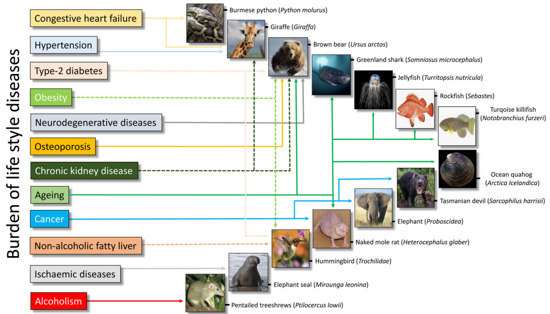
Figure 2: Examples of species that already have been identified as being of interest for finding novel targets for “burden of life style” diseases that accumulate as we get older. Among a number of diseases that often tend to cluster (diseasome), studies of some species in nature have already provided some clues for better treatment of congestive heart failure, hypertension, type-2 diabetes, obesity, neurodegenerative diseases, osteoporosis, chronic kidney disease, ageing, cancer, non-alcoholic fatty liver, ischaemic diseases (such as acute kidney injury) and alcoholism.
