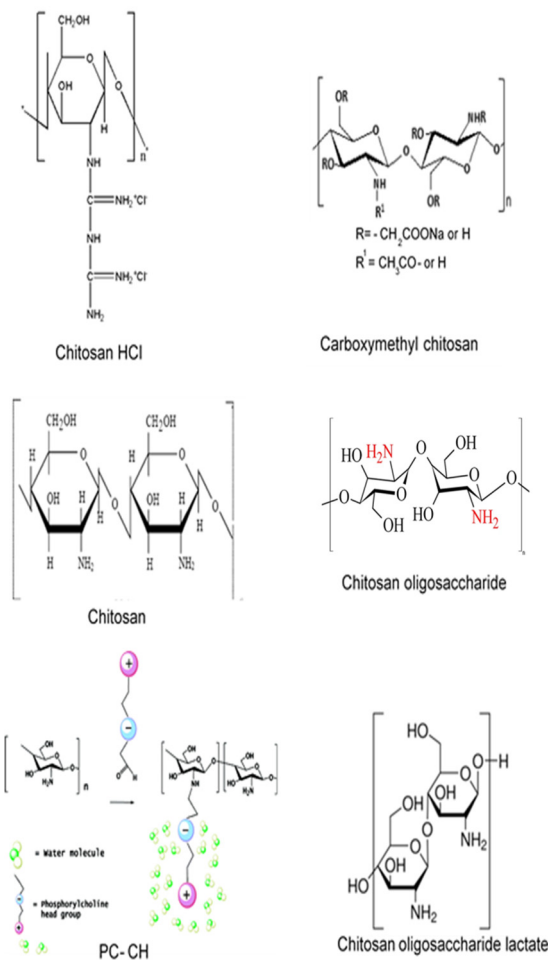
FIG 8 The structures of chitosan (60) and its derivatives, chitosan HCl, carboxymethyl chitosan (61), chitosan oligosaccharide (60), PC-chitosan (republished from reference 28 with permission of the publisher), and chitosan oligosaccharide lactate (59).
