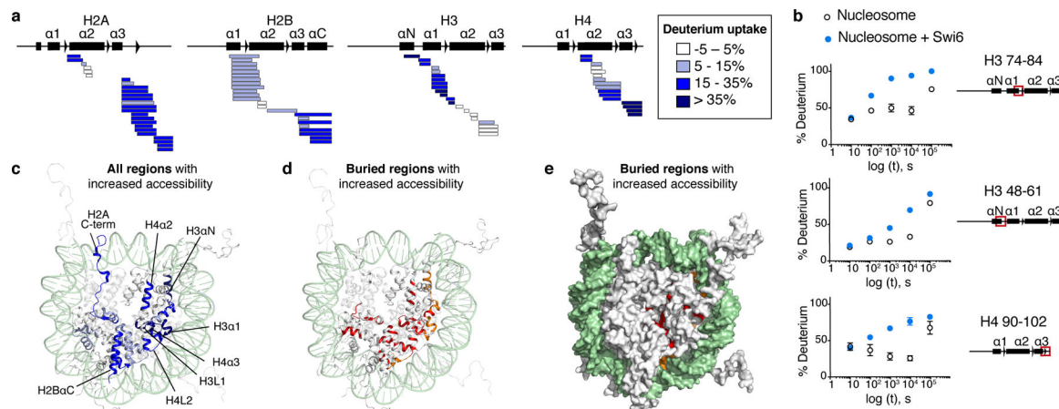
Fig. 2: Swi6 binding increases solvent accessibility of buried histone residues. (a) Differential HDX-MS of individual histones within Swi6-bound versus free nucleosomes from a single time point ( 10^4 sec; all time points in Extended Data Fig. 3). Each horizontal bar represents an individual peptide. Peptides are placed beneath schematic of secondary structure elements. Color map represents percent increase in deuterium uptake observed upon Swi6 binding. The percent increase values are derived from multiple peptides obtained from one of two independent experiments with similar results. (b) Kinetics of deuterium uptake of example histone peptides (residue numbers indicated) over time. Data are mean and SD of multiple peptides obtained from one of two independent experiments with similar results. Error bars not shown for points when shorter than the height of the symbol. (c) Histones in nucleosome structure (PDB 1KX5) colored according to the percent of deprotection in (a). For clarity, only one copy of histones is colored. DNA is in light green. (d) Buried regions showing increase in deuterium uptake upon Swi6 binding are highlighted in ribbon diagram. Residues proximal to DNA and histones are in orange and red, respectively. (e) Residues in (d) shown in space-fill representation.
