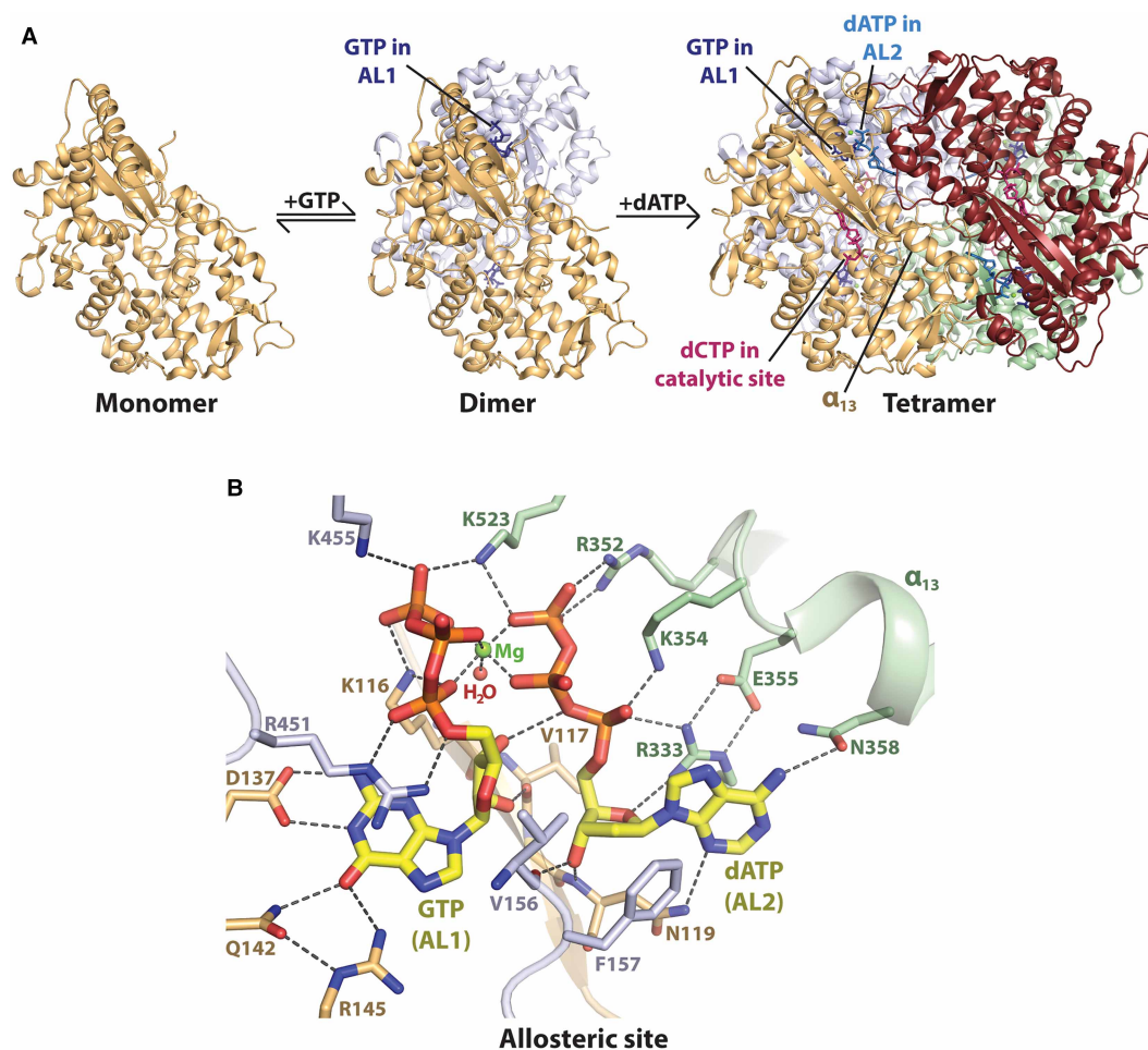
Figure 2. Nucleotide-dependent tetramerization of SAMHD1 HD domain.
