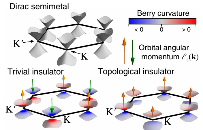
Fig. 1. Illustration of the Berry curvature and orbital angular momentum. The surfaces represent the valence and conduction band, while the coloring indicates the Berry curvature. The arrows illustrate the orbital angular momentum of the valence band.
