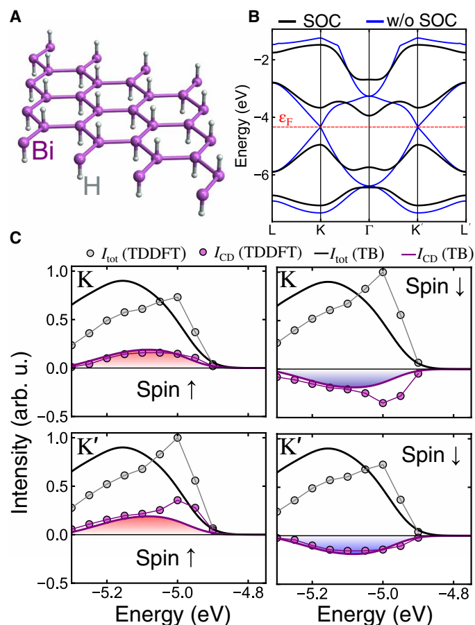
Fig. 4. Circular dichroism in BiH. (A) Lattice structure of hexagonal BiH. (B) Band structure of hydrogenated bismuthane (BiH; obtained from DFT), fully including SOC (black) and, for the purpose of comparison, without any SOC (blue lines). (C) Integrated dichroic signal as in Fig. 2 for spin-up (left panels) and spin-down (right panels) electrons at K (top panels) and K' (bottom panels), respectively.
