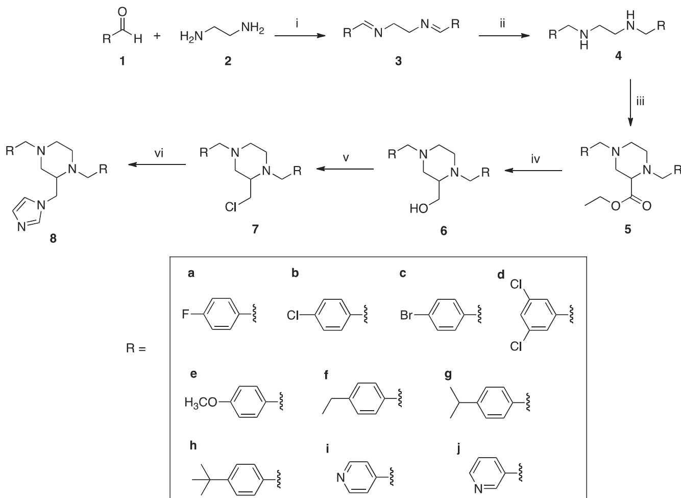
Scheme 1. Reagents and conditions: (i) EtOH, r.t., o/n (ii) \text{NaBH}_4 , MeOH, r.t., 4 h (iii) \text{Et}_3\text{N} , 2,3-dibromopropionic acid ethyl ester, toluene, 80 ^\circ\text{C} , o/n (iv) \text{LiAlH}_4 , THF, r.t., o/n (v) \text{SOCl}_2 , \text{CH}_2\text{Cl}_2 , r.t., 48 h (vi) (a) Imidazole, \text{K}_2\text{CO}_3 , \text{CH}_3\text{CN} , 45 ^\circ\text{C} , 1 h (b) chloride 7, 70 ^\circ\text{C} , 48 h.
