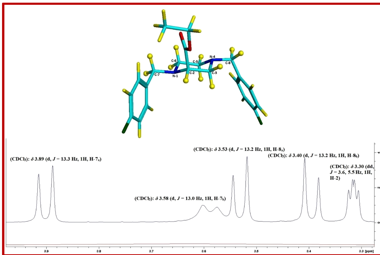
Fig. 3. Ethyl 1,4-bis(4-fluorobenzyl)piperazine-2-carboxylate ( 5a ) chair conformation with vicinal and geminal couplings of H-2, H-7 and H-8 protons.
