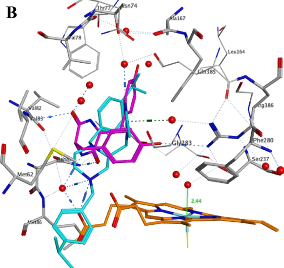
Fig. 6. Docking of representative piperazines (cyan) (A) 8b in binding mode 1 and (B) 8g in binding mode 2 in the CYP121A1 active site compared with cYY (magenta). [Haem (orange), water molecules (red spheres)].
