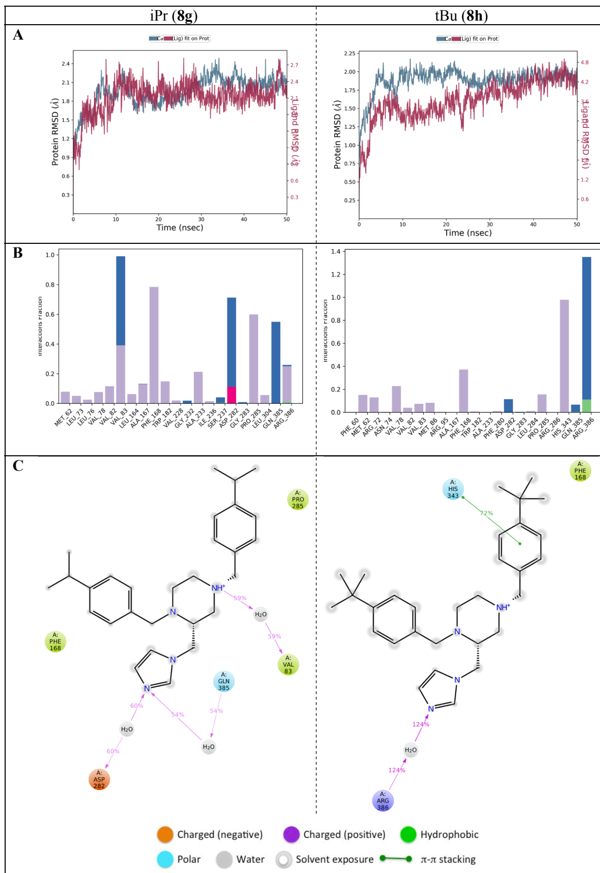
Fig. 7. (A) Protein (blue) and ligand (red) root mean square of the CYP121A1- 8g and 8h complexes (B) Illustration of protein interactions with the ligand. The red column means ionic bond, green column a hydrogen bond, blue column water bridges, and a purple column a hydrophobic bond. The stacked bar charts are normalised over the course of the trajectory: for example, a value of 0.5 suggests that for 50% of the simulation time, the specific interaction is maintained (C) A schematic of detailed ligand atom interactions with the protein residues. Interactions that occur > 30.0% of the simulation time in the selected trajectory (0.00 through 50.05 nsec), are shown (note: it is possible to have interactions with > 100% as some residues may have multiple interactions of a single type with the same ligand atom e.g. the ARG side chain has four H-bond donors that can all hydrogen-bond to a single H-bond acceptor).
