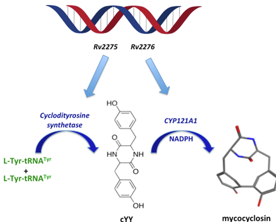
Fig. 1. Cyclodityrosine synthetase and CYP121A1 reactions to produce the cyclic dipeptide, cyclo-L-Tyr-L-Tyr (cYY), and the novel secondary metabolite mycocyclusin.
