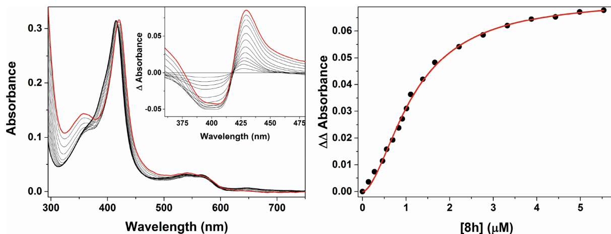
Fig. 5. UV-Vis optical binding titration for compound 8h binding to CYP121A1. The left hand panel shows data from a compound 8h titration with CYP121A1 ( \sim 4.7 \mu\text{M} ) with the ligand-free spectrum as a thick black line, spectra following progressive additions of 8h as thin solid lines, and the final near-saturated protein spectrum shown as a thick red line. The inset shows overlaid difference spectra generated by the subtraction of the starting spectrum from each consecutive ligand-bound spectrum collected in the titration. The right hand panel shows a plot of compound 8h -induced absorbance change – calculated as the difference between the peak and trough in the difference spectra in the left hand panel, using the same wavelength pair (429 and 392 nm, respectively) throughout. Data were fitted using the Hill equation to give a 8h K_D value of 1.2 \pm 0.1 \mu\text{M} .
