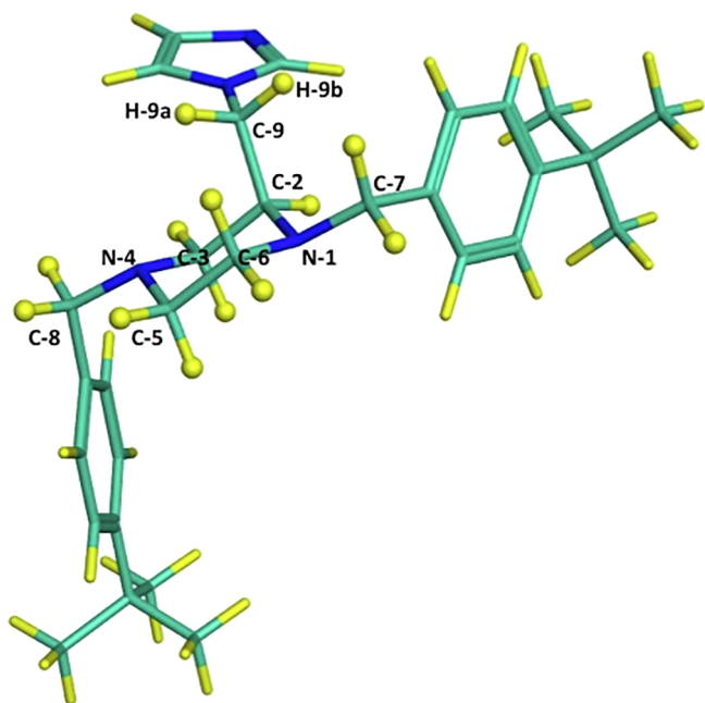
Fig. 4. 2-((1H-Imidazol-1-yl)methyl)-1,4-bis(4- tert -butylbenzyl)piperazine ( 8h ) chair conformation after energy minimisations to explain vicinal and geminal couplings between H-9, H-2, H-7, H-8 protons.
