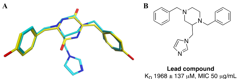
Fig. 2. (A) Flexible alignment of cYY (yellow) and lead compound (cyan) showing overlap (B) Binding affinity and MIC data for lead compound.
