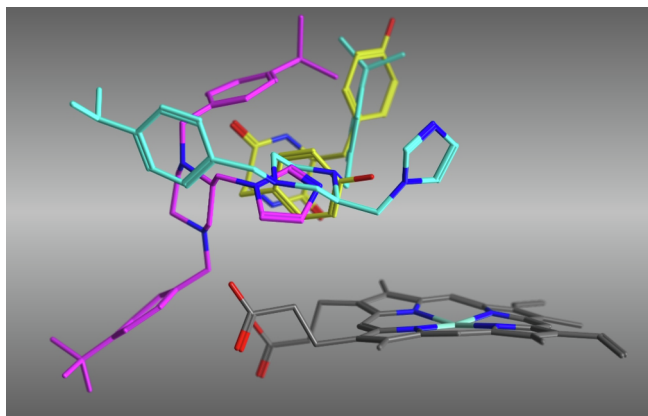
Fig. 8. Positioning of the isopropyl derivative ( 8g , cyan) and tert -butyl derivative ( 8h , magenta) compared with cYY (yellow) after molecular dynamics simulation.
