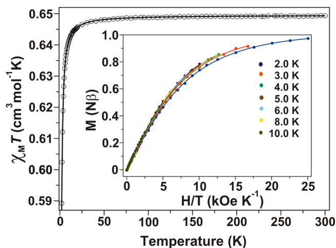
Figure 2. Magnetometry of CrW 12 . Temperature dependence of \chi_M T and the magnetization curves (inset) for CrW 12 : (O, ●) experimental; (—) best-fit curves to the experimental data using the parameters provided in the text. The \chi_M T value supports a partial (36%) occupancy of Cr III .
