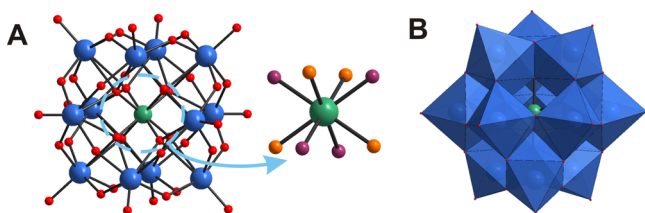
Figure 1. CrW 12 anion. (A) Ball-and-stick representation including the crystallographic disorder in {CrO 4 }. (B) Polyhedral representation. Color code: W, blue; Cr, green; O, red, orange, and purple.
