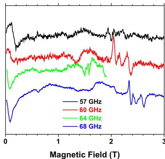
Figure 3. HFEPFR spectra of CrW 12 at 4.5 K and indicated frequencies in the vicinity of the zero-field transition between the \pm 1/2 and \pm 3/2 Kramers doublets. The resonances appearing between 2 and 3 T depending on frequency ( g \sim 1.95 ) belong to a different spin species, which has a much lower anisotropy (about 0.1 cm -1 ) and thus represents a small fraction of total absorption despite its amplitude, signifying low abundance.
