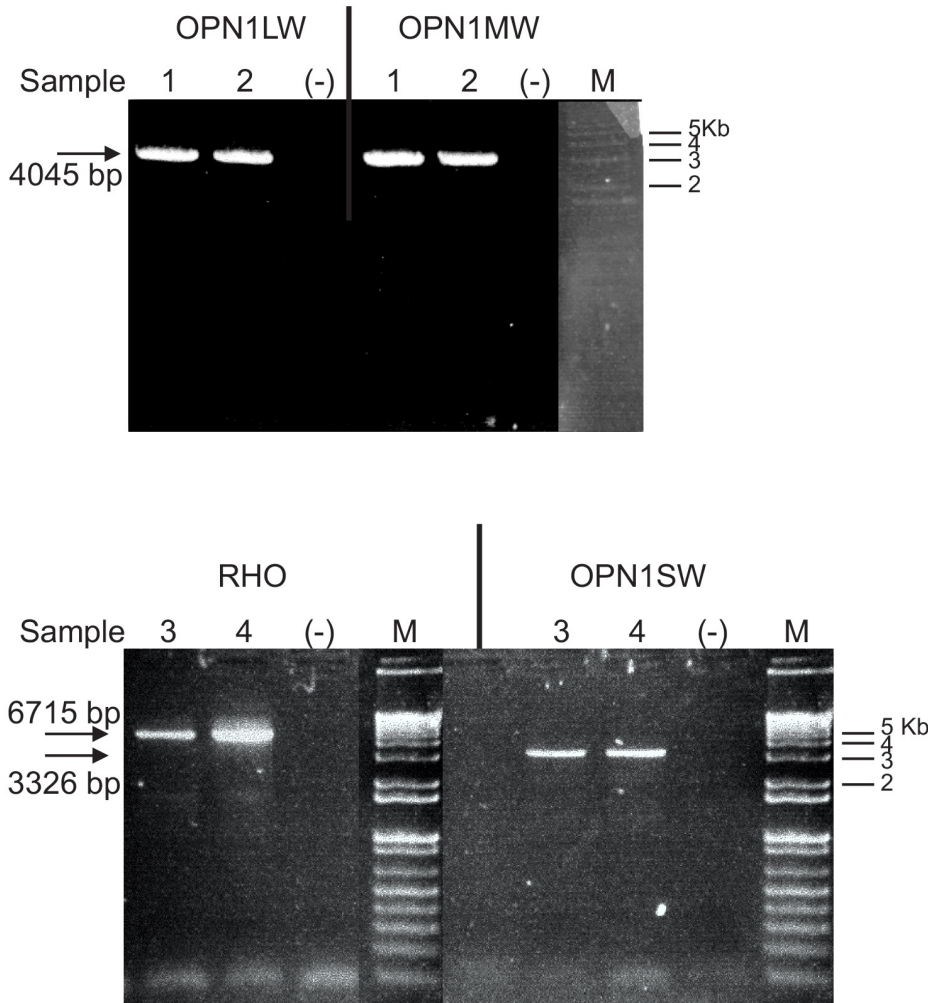
Figure 1. Representative gel images of OPNILW , OPNIMW , RHO , and OPNISW PCR products. The first gel image represents the PCR products of OPNILW and OPNIMW from two subjects. The size of both PCR products is 4,045 bp. M = DNA ladder. The DNA ladder positions are identified at 5, 4, 3, and 2 kb. The second gel image represents the PCR products of RHO and OPNISW in subjects 3 and 4. The RHO PCR product is 6,715 bp. The OPNISW PCR product is 3,326 bp.
