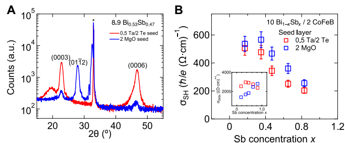
Fig. 4. Facet dependence of \sigma_{\text{SH}} . (A) XRD spectra for 8.9 \text{Bi}_{0.53}\text{Sb}_{0.47} grown on 0.5 Ta/2 Te (red) and 2 MgO (blue) seed layers. Heterostructures without the CoFeB layer were used. (B) Sb concentration ( x ) dependence of SHC \sigma_{\text{SH}} for 10 \text{Bi}_{1-x}\text{Sb}_x/2 CoFeB heterostructures with the two seed layers described in (A). The inset shows the x dependence of \sigma_{\text{BiSb}} . The measurement temperature is 300 K.
