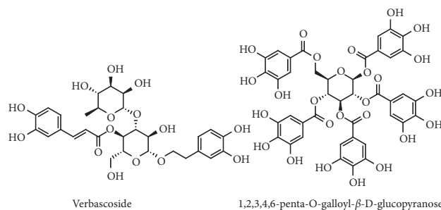
FIGURE 13: Structures of verbascoside and 1,2,3,4,6-penta-O-galloyl- \beta -D-glucopyranose.
