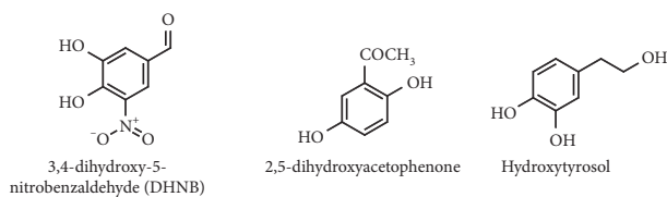
FIGURE 11: Structures of simple phenolic compounds with XO inhibitory activity and decreasing effect of serum UA levels.
