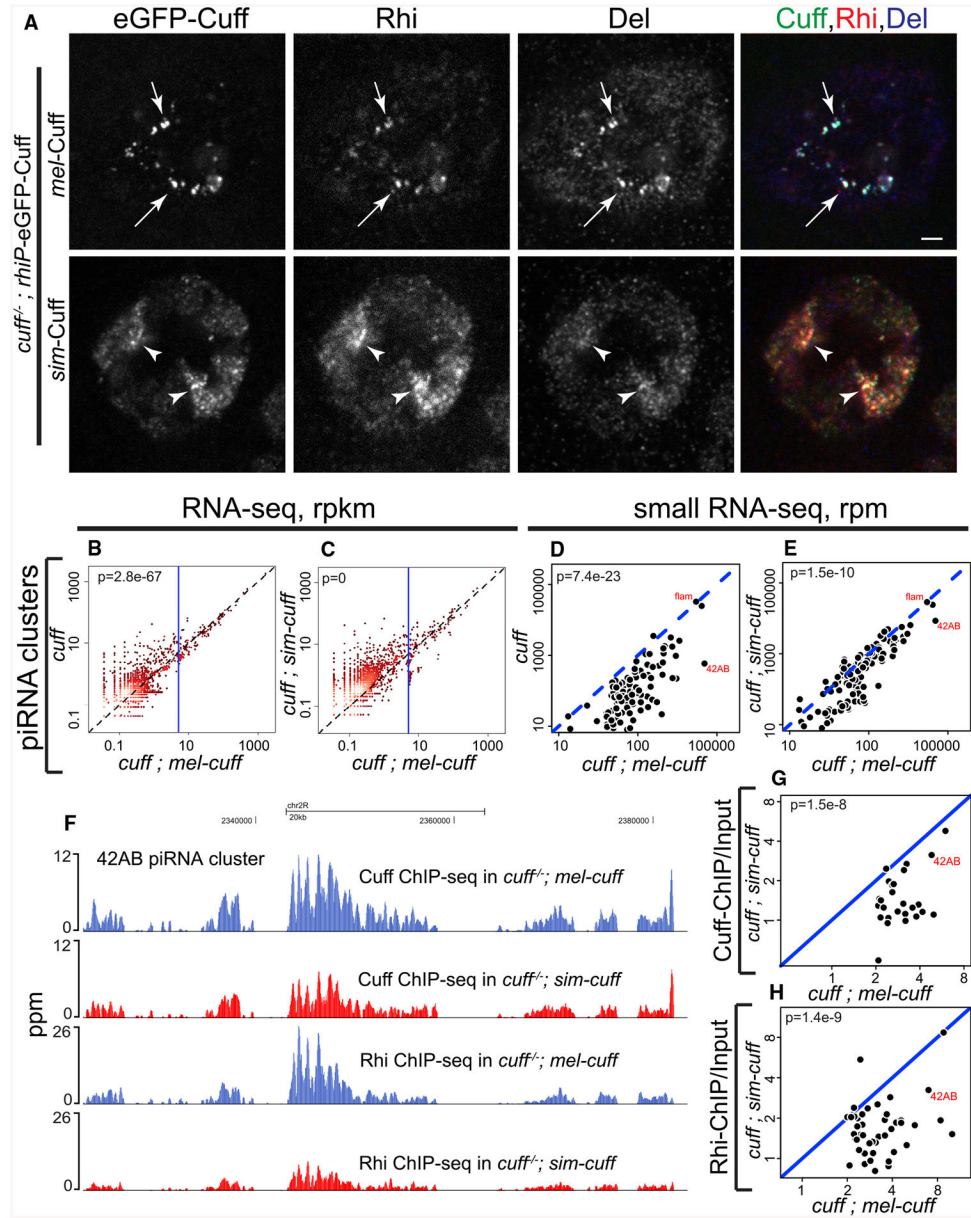
Figure 2. sim -Cuff Disrupts RDC Localization
