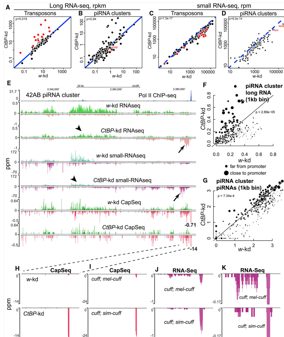
Figure 4. CtBP Suppresses Canonical Transcription at piRNA Clusters
