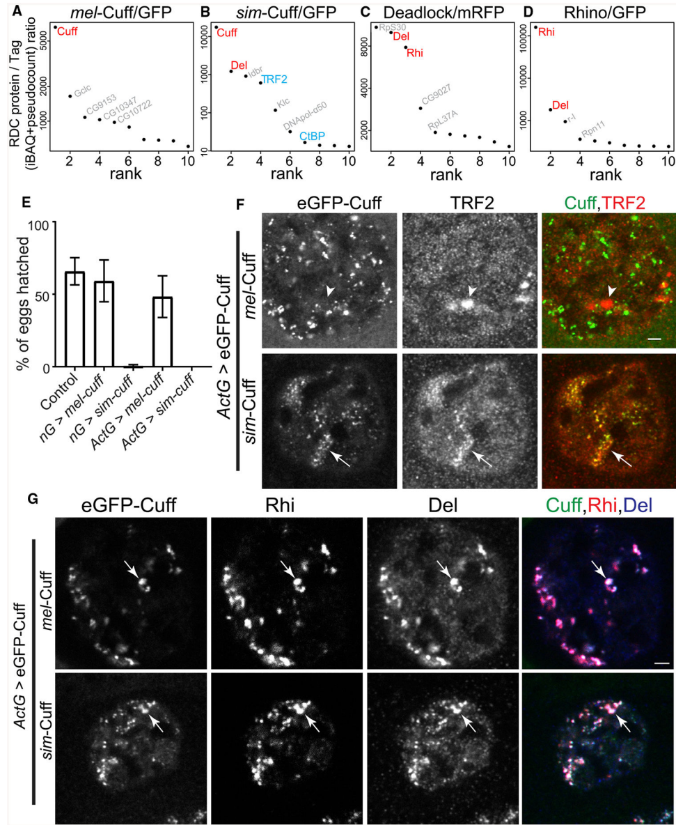
Figure 3. D. simulans Cuff Traps Transcription Factors and Acts as a Dominant Negative (A–D) Mass spectrometric analysis of mel -Cuff (A), sim -Cuff (B), Del (C), and Rhino (D) binding proteins. Graphs show ratios of iBAQ value of a bound protein in a RDC protein IP versus tag control IP ranked by ratio values. RDC components are shown in red, TRF2 and CtBP in blue.
