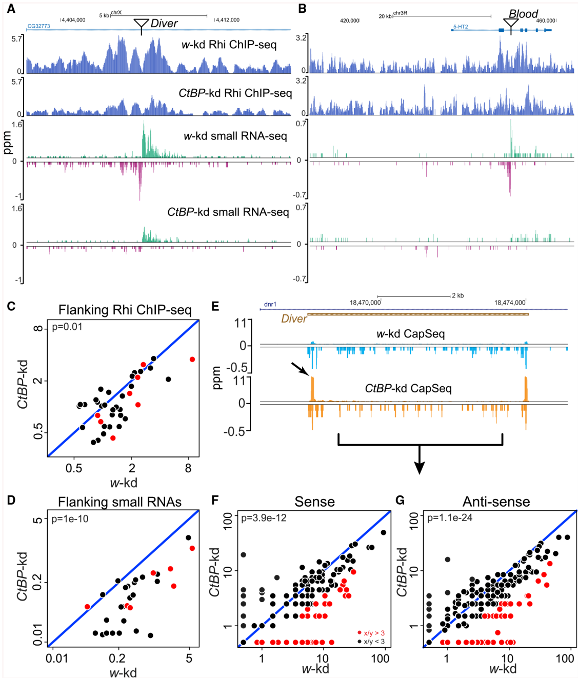
Figure 5. CtBP Suppresses Canonical Transcription of Dispersed Transposon Insertions (A and B) Genome Browser views of Rhi ChIP-seq and small RNA-seq profiles flanking dispersed transposons, Diver (A) and Blood (B), in CtBP-kd and w-kd . The transposon insertion is shown at the top. (C and D) Scatterplots showing comparisons of RPM values of Rhi ChIP-seq (C) and small RNAs (D), 0.5 kb upstream and downstream of new transposons in CtBP-kd versus w-kd . The transposons insertions were identified by genomic sequencing with TEMP (Zhuang et al., 2014), and the graphs show the values for new TEs (not present in the reference genome), which have both flanking piRNAs and Rhi signal. Red points denote expression of
