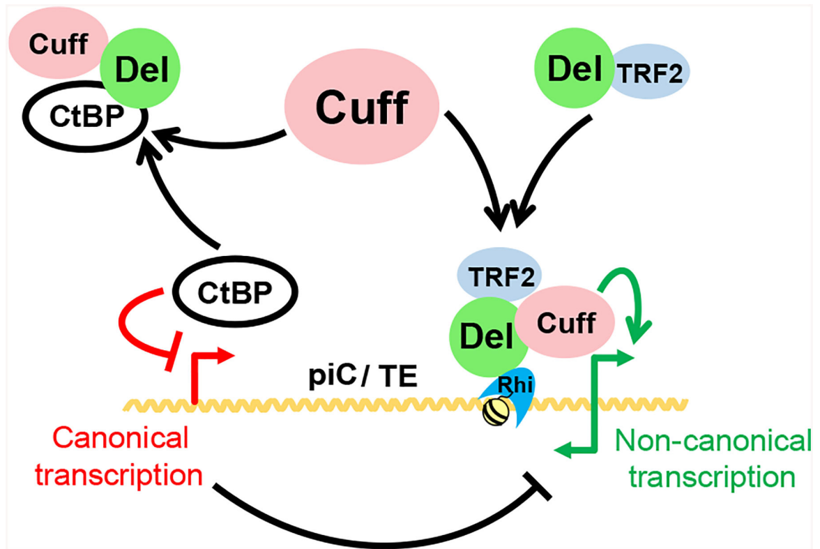
Figure 7. Model for a Transcriptional Network Balancing Canonical and Non-canonical piRNA Precursor Transcription
