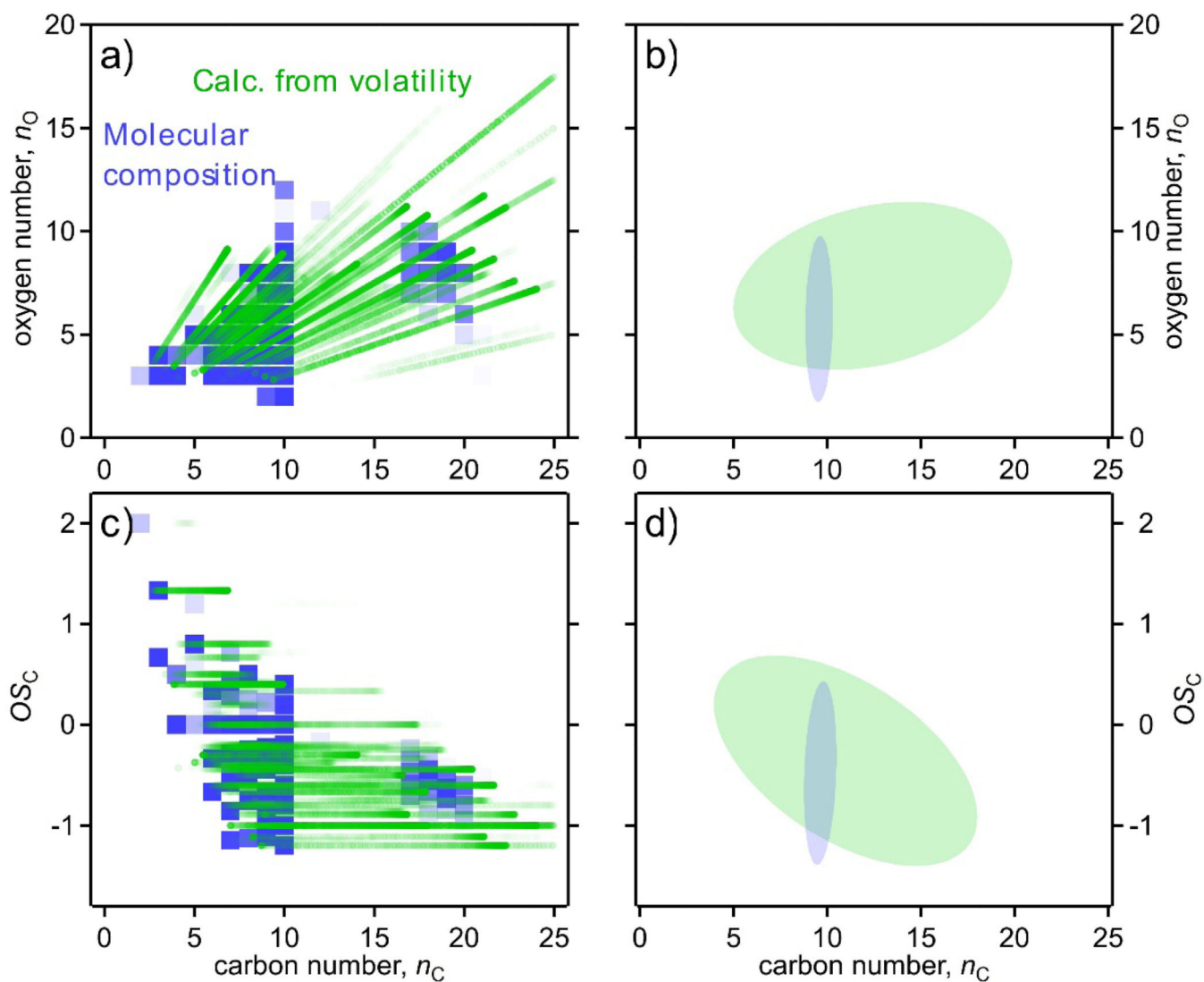
Figure 3. Comparison of distribution of FIGAERO I - CIMS in two frameworks: (a,b) oxygen number by carbon number, and (c,d) oxidation state of carbon by carbon number. Directly measured parameters from molecular formulas ( n_C, n_O ) are blue (squares). Parameters calculated from volatility based on Eqs. 2 and 4 ( n_{C,calc}, n_{O,calc} ) are green (dots). Left: individual ions shown, opacity proportional to measured mass. Right: ovals that contain 80% of measured instrument mass (optimized as smallest area ellipse that meets this criteria).
