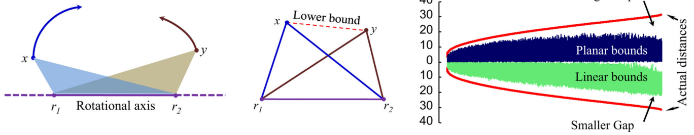
Fig. 9. (Left) Two points x and y are projected on a plane by a rotation around the axis joining two reference points r_1 and r_2 . (Mid) Known distances and the lower bound after the projection. (Right) Planar and linear bound are plotted against true distances for 40,000 random pairs
