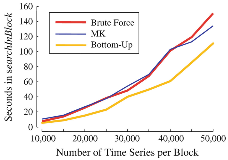
Fig. 8. Comparison of in-memory search methods
