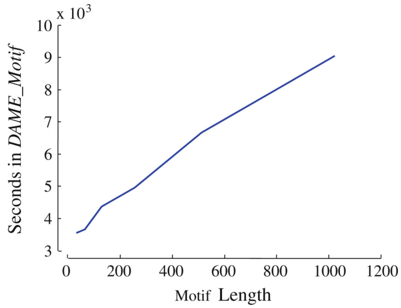
Fig. 7. Execution times on one million random walks of different lengths
