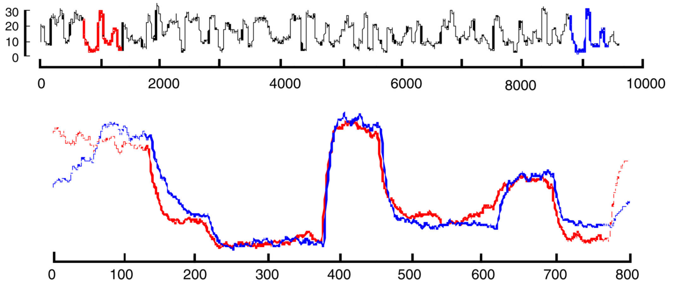
Fig. 1. ( Top ) The output steam flow telemetry of the Steamgen dataset has a motif of length 640 beginning at locations 589 and 8,895. ( Bottom ) By overlaying the two motifs we can see how remarkably similar they are to each other
