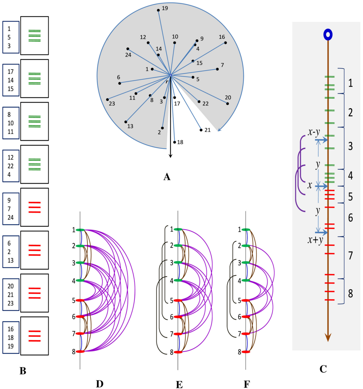
Fig. 3. a A sample database of 24 points. b Disk blocks containing the points sorted in the order of the distances from r . The numbers on the left are the ids. c All points projected on the order line . d A portion of an order line for a block of 8 points. e After pruning by a current motif distance of 4.0 units. f After pruning by 3.0 units
