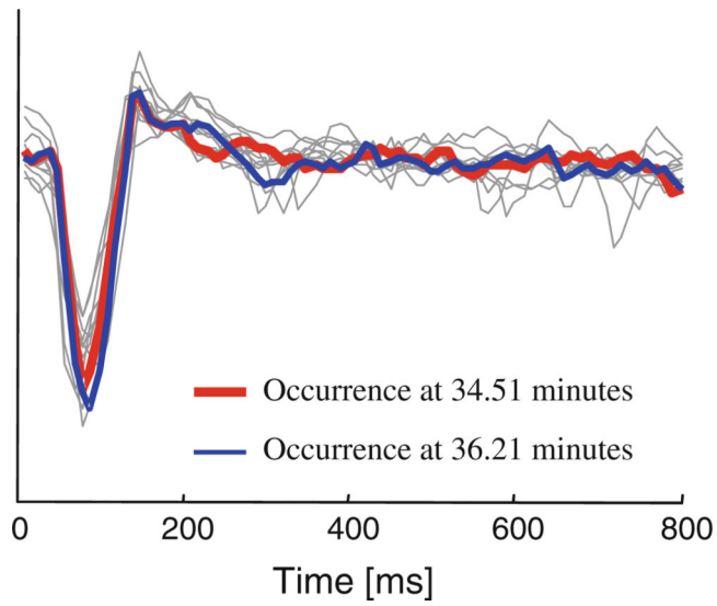
Fig. 18. (Left) Bold lines the first motif found in one hour of EEG trace LSF5. Light lines the ten nearest neighbors to the motif. (Right) A screen dump of Fig. 6, from paper Stefanovic et al. (2007)
