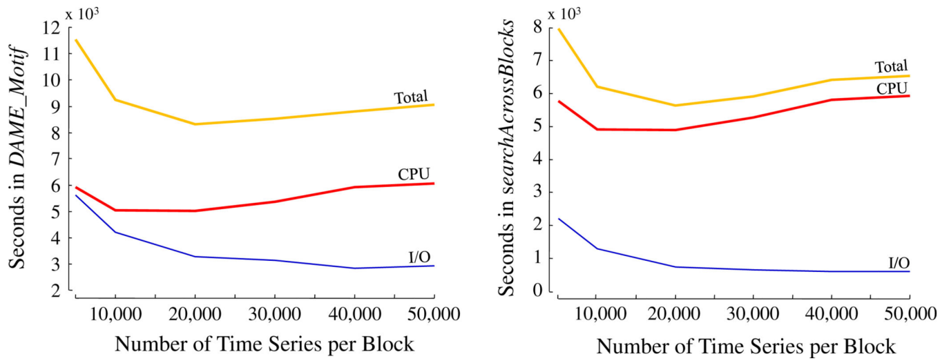
Fig. 6. Total execution times with CPU and I/O components recorded on one million random walks for different block sizes ( left ) for the DAME_Motif method and ( right ) for the searchAcrossBlocks method
