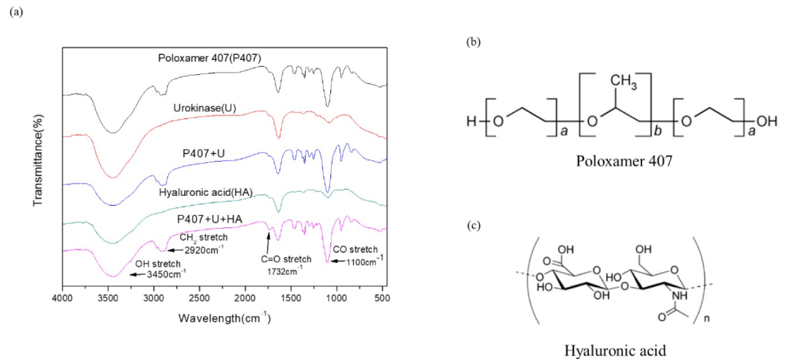
Fig 1. FT-IR spectra (a) of aqueous P407, U, P407+U, HA, and P407+U+HA. Chemical structure of (b) P407 and (c) HA.
