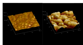
AFM phase images showing alginate films. Images are 300 nm in x and y and 35° in z. Left: control alginate films without CHX-HMP. Right: Alginate films with embedded CHX-HMP particles.
