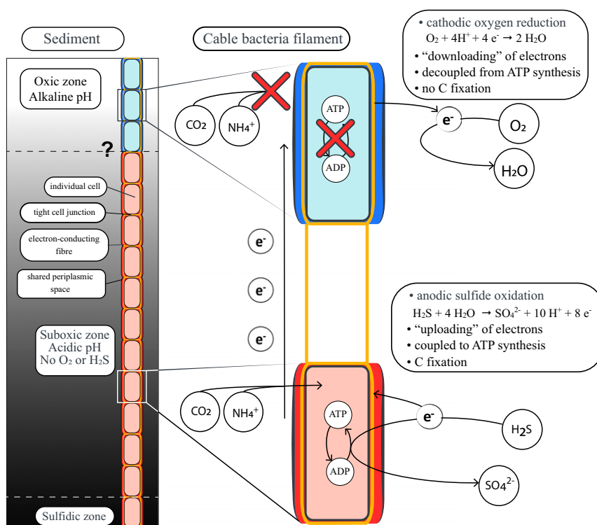
Fig. 4. Schematic representation of the energy metabolism of a cable bacterium. The cells in the suboxic and sulfidic zone (red) perform anodic H 2 S oxidation. The free energy released by this redox half-reaction is utilized for generating ATP, thus allowing the assimilation of carbon and nitrogen, while the generated electrons are transported toward cells in the oxidic zone via conductive fibers in the shared periplasmic space. Cells in the oxidic zone (blue) utilize these electrons to perform cathodic O 2 reduction, but this results in very little to no release of free energy and hence no capacity to assimilate carbon and ammonia.
